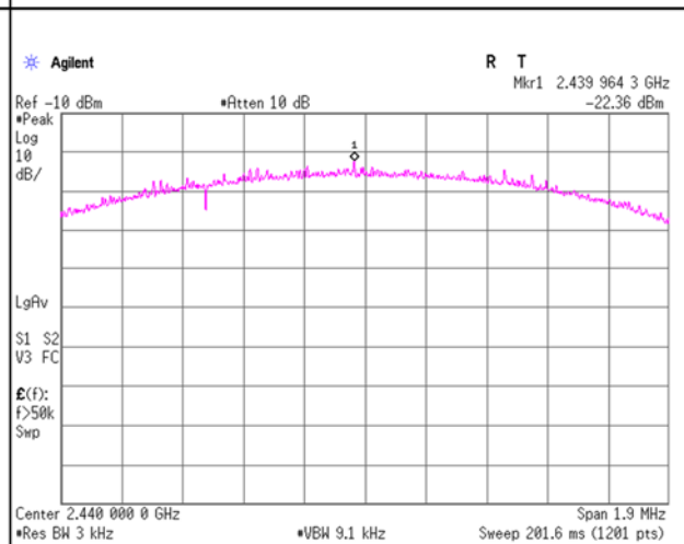
2440 MHz
