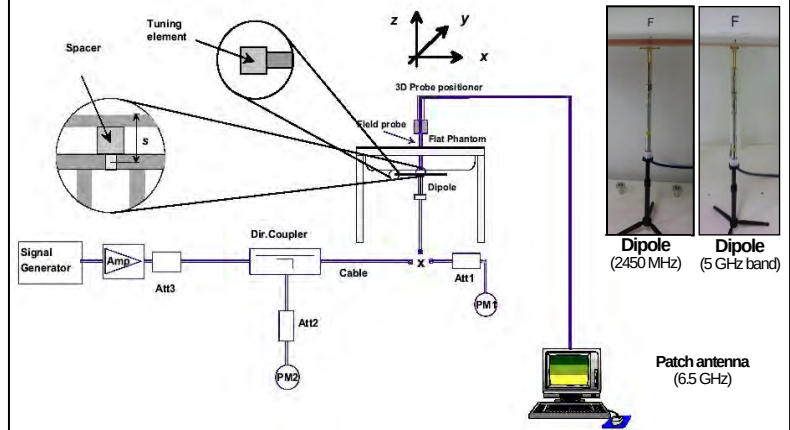
Figure. Test setup for the system performance check (example)
