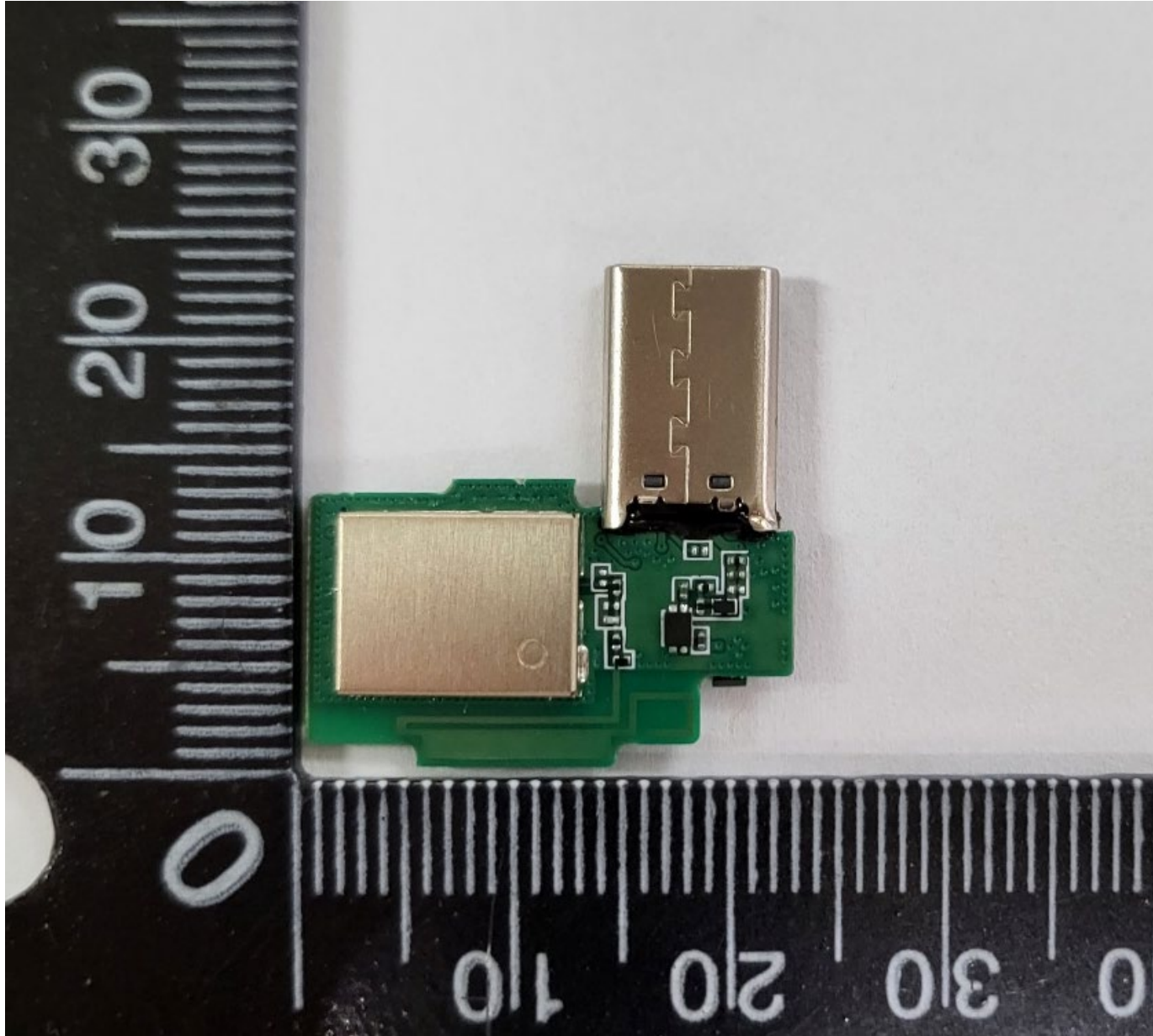
USB Transceiver _ Pattern Antenna
