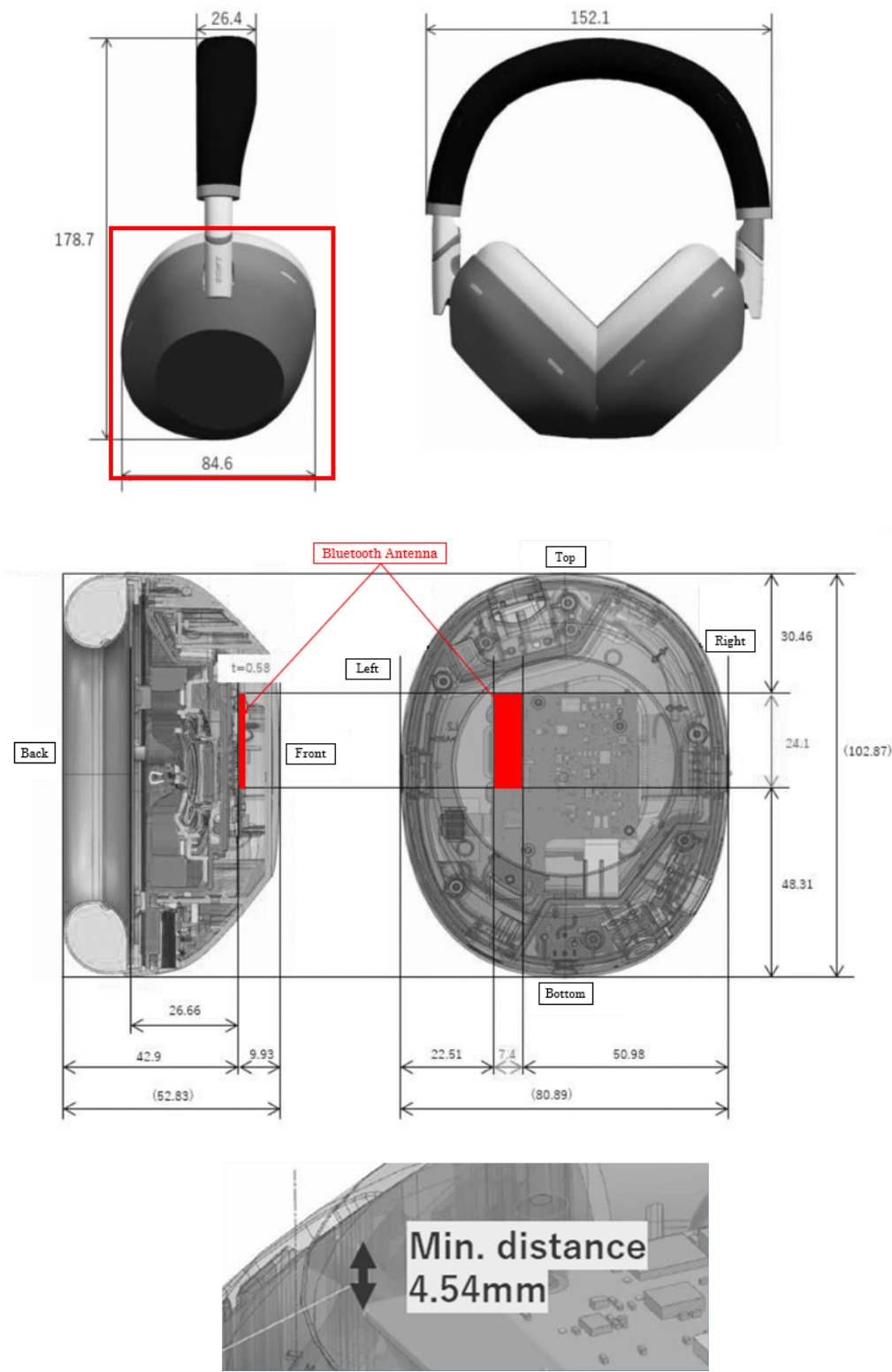
Figure D-5 Antenna Dimensions and Separation Distances
