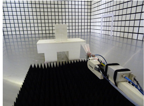
Above 1 GHz
