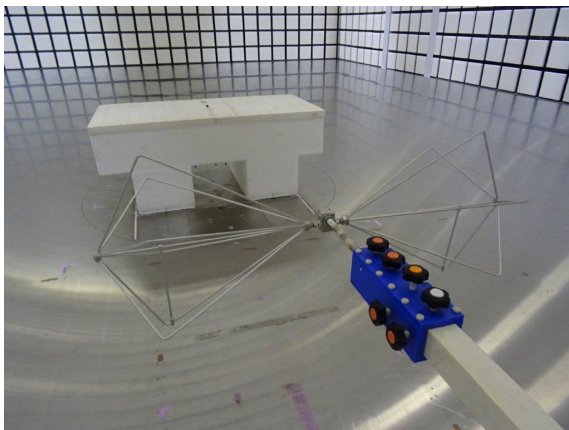
Below 1 GHz
