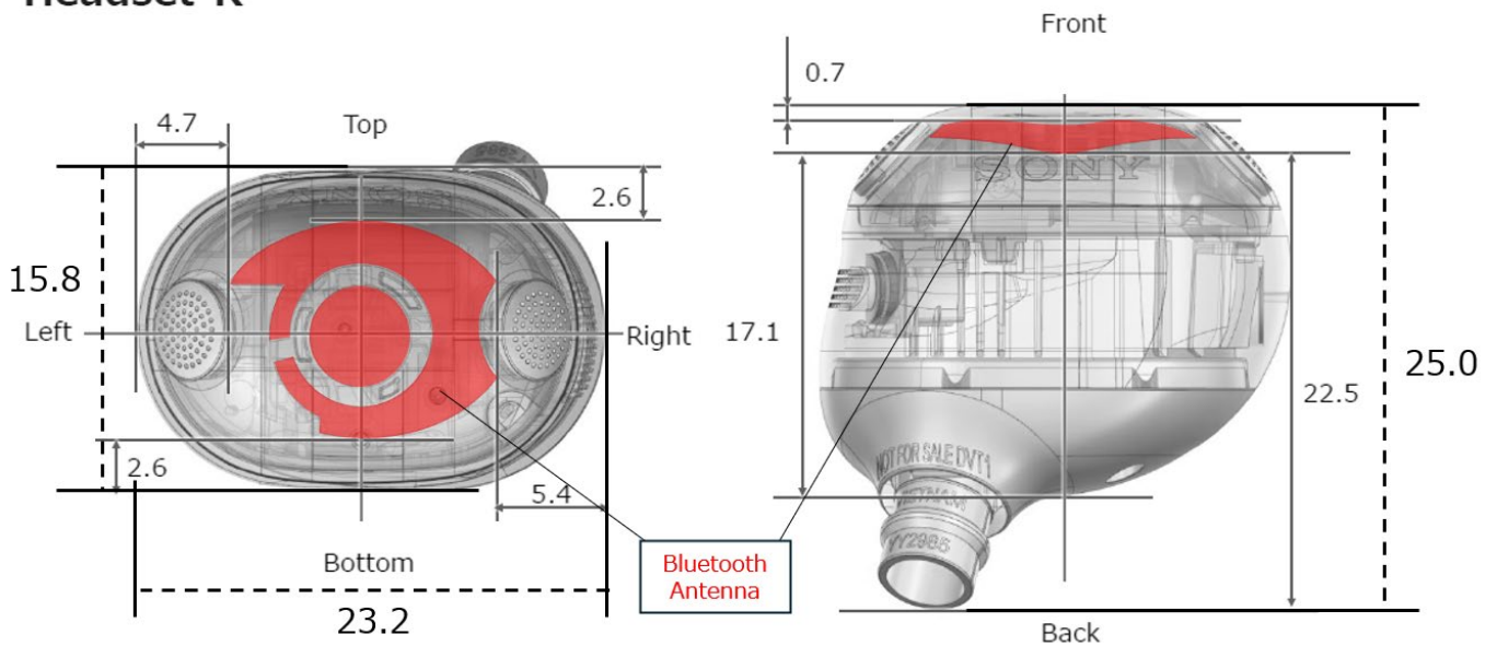
Figure D-13 Antenna Dimensions and Separation Distances
