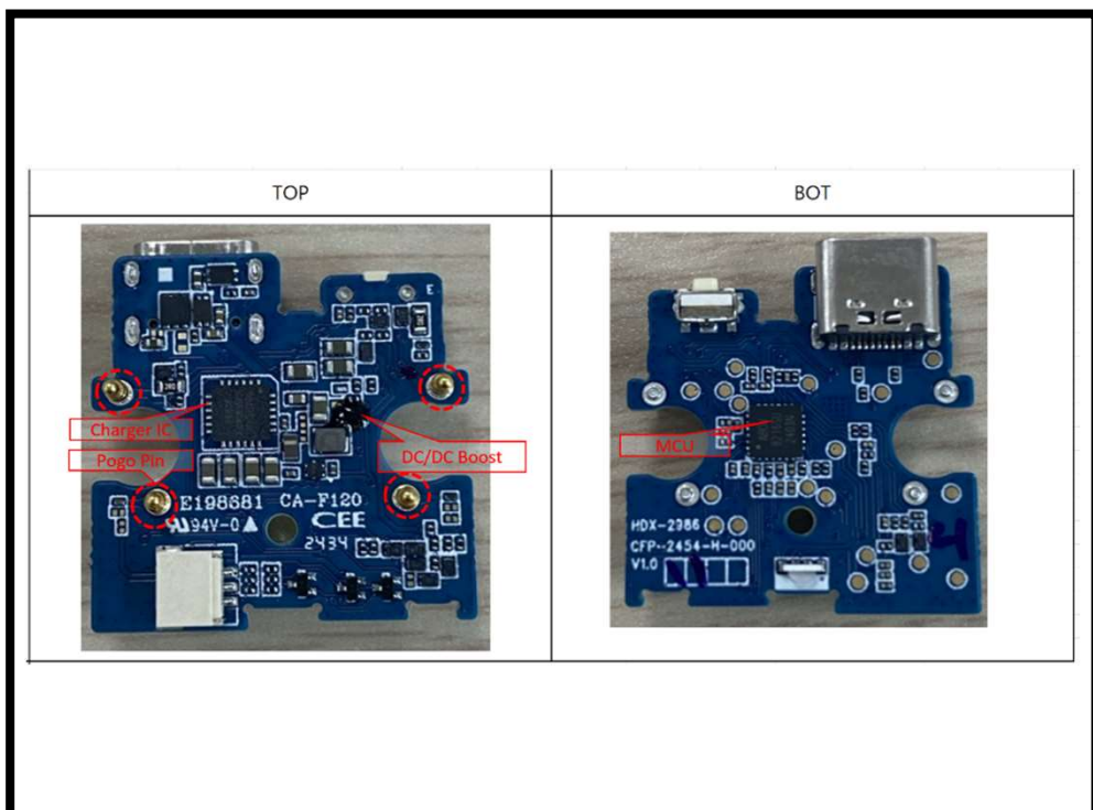
Charging Case Main Board Internal View
