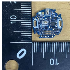
Earbuds L-CH Board
