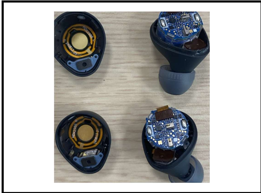
L/R Earphone Internal View
