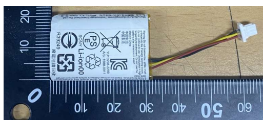
Case Battery (High-Power)
