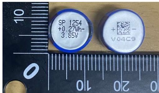
Earbuds Battery (High-Power)
