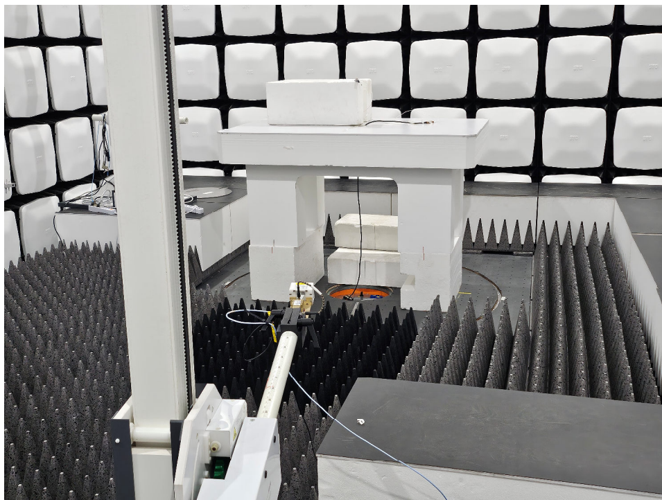
18 GHz Above
