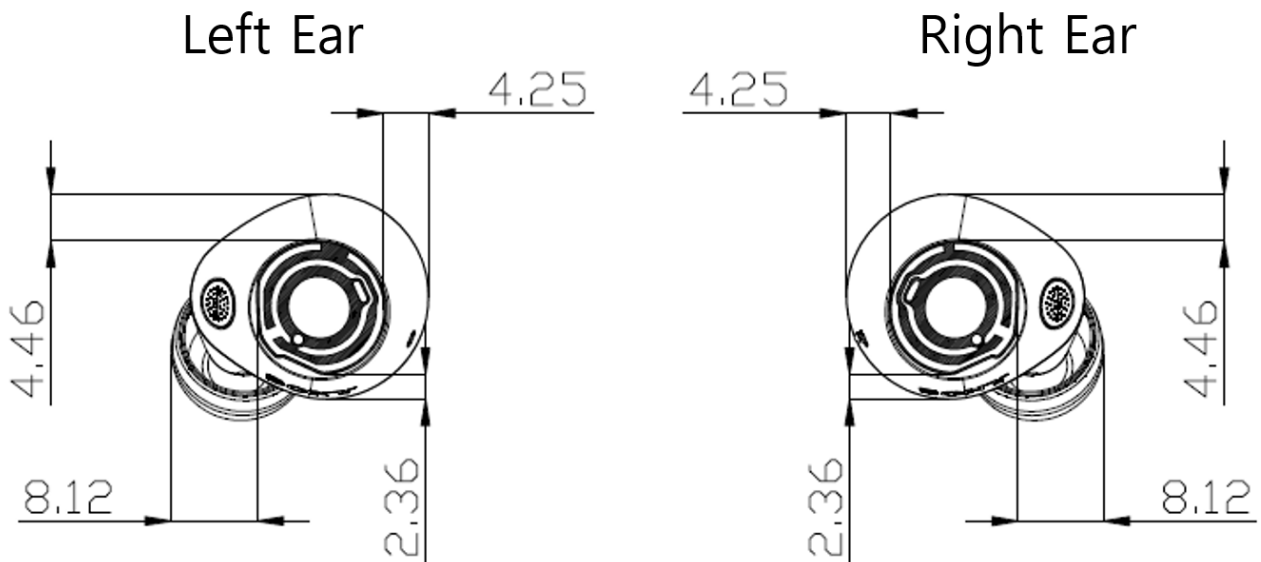
Figure E-1 Antenna Location (Rear Side View)
