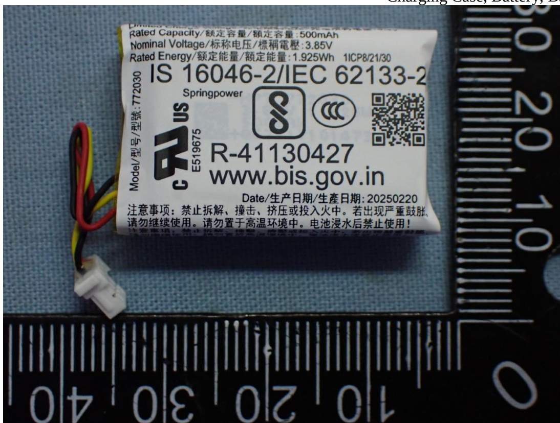
Figure 44 Charging Case, Battery, Back View
