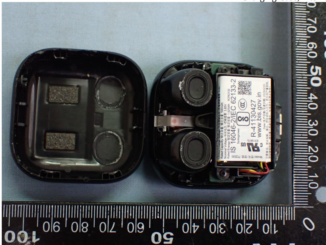
Figure 38 Charging Case, Internal View
