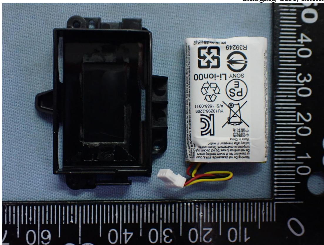
Figure 41 Charging Case, Internal View
