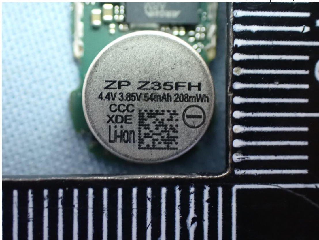
Figure 34 Left Earphone, Battery View
