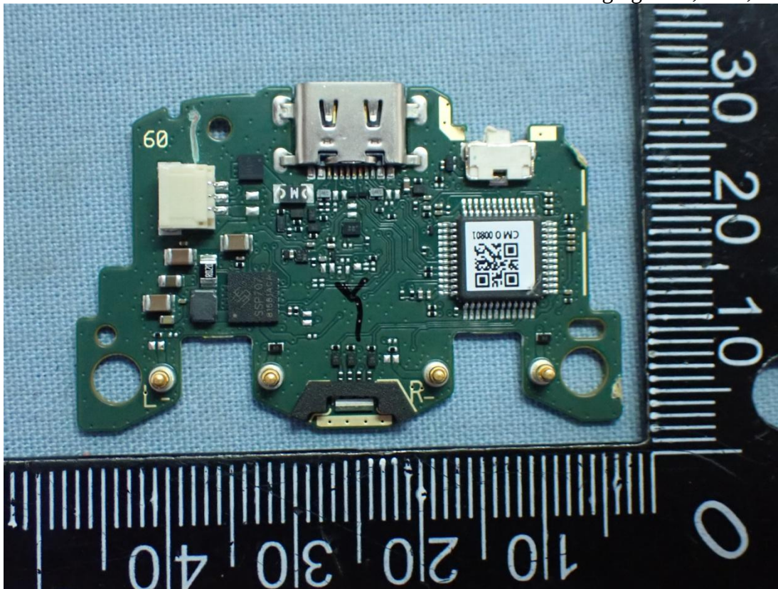
Figure 45 Charging Case, PCB, Front View
