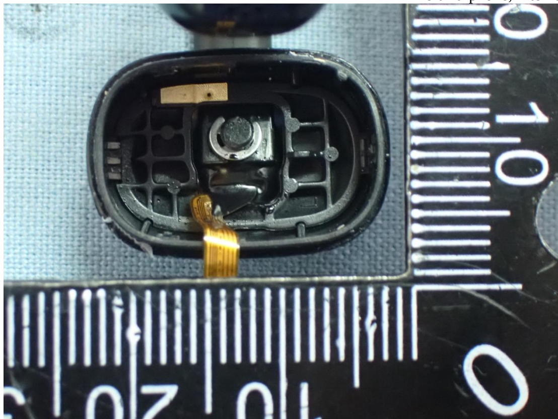
Figure 30 Left Earphone, Internal View
