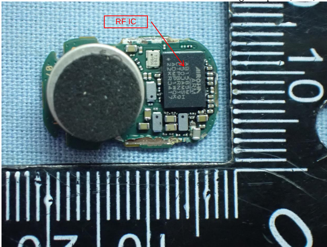
Figure 27 Right Earphone, PCB, Front View
