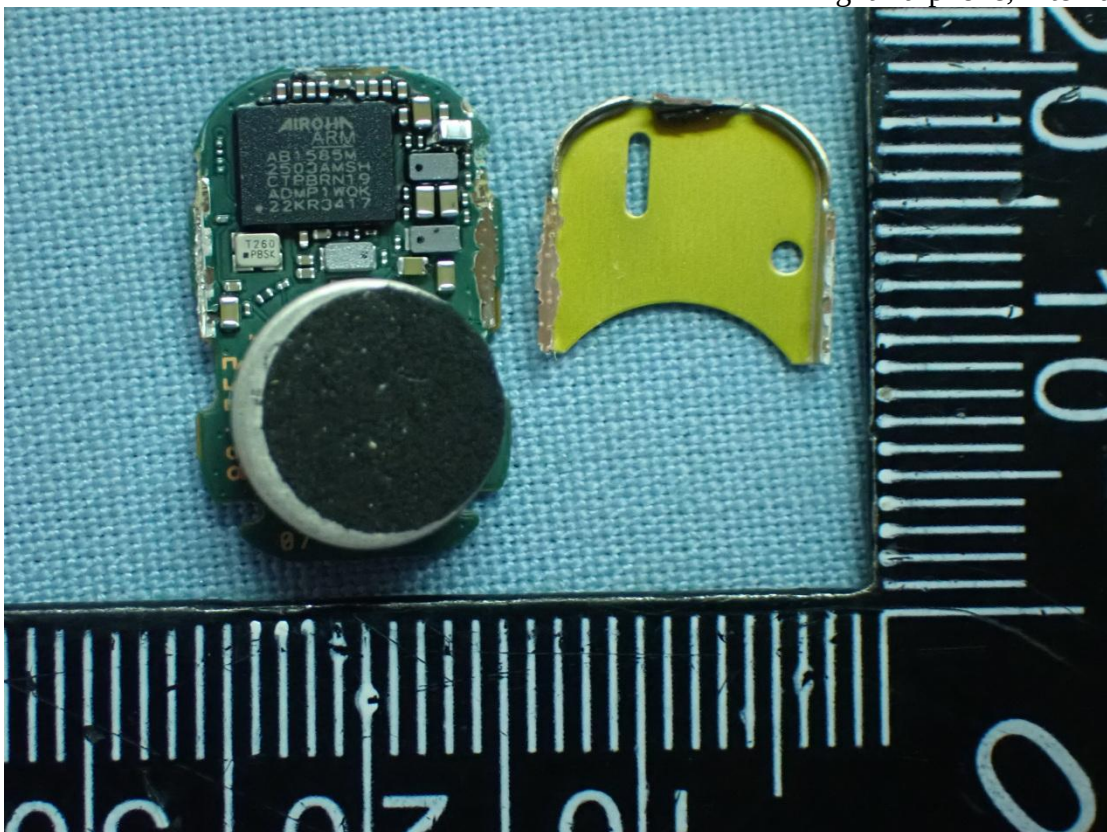
Figure 24 Right Earphone, Internal View
