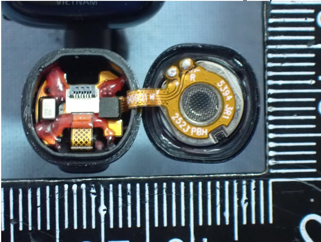
Figure 26 Right Earphone, Battery View
