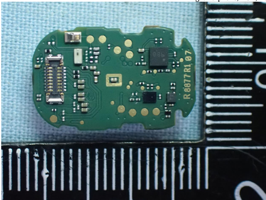
Figure 28 Right Earphone, PCB, Back View
