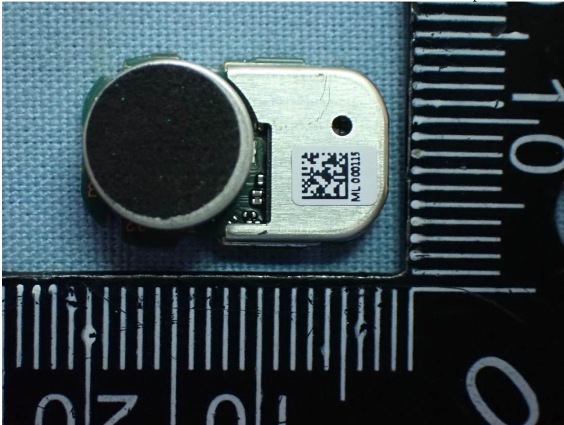
Figure 32 Left Earphone, Internal View
