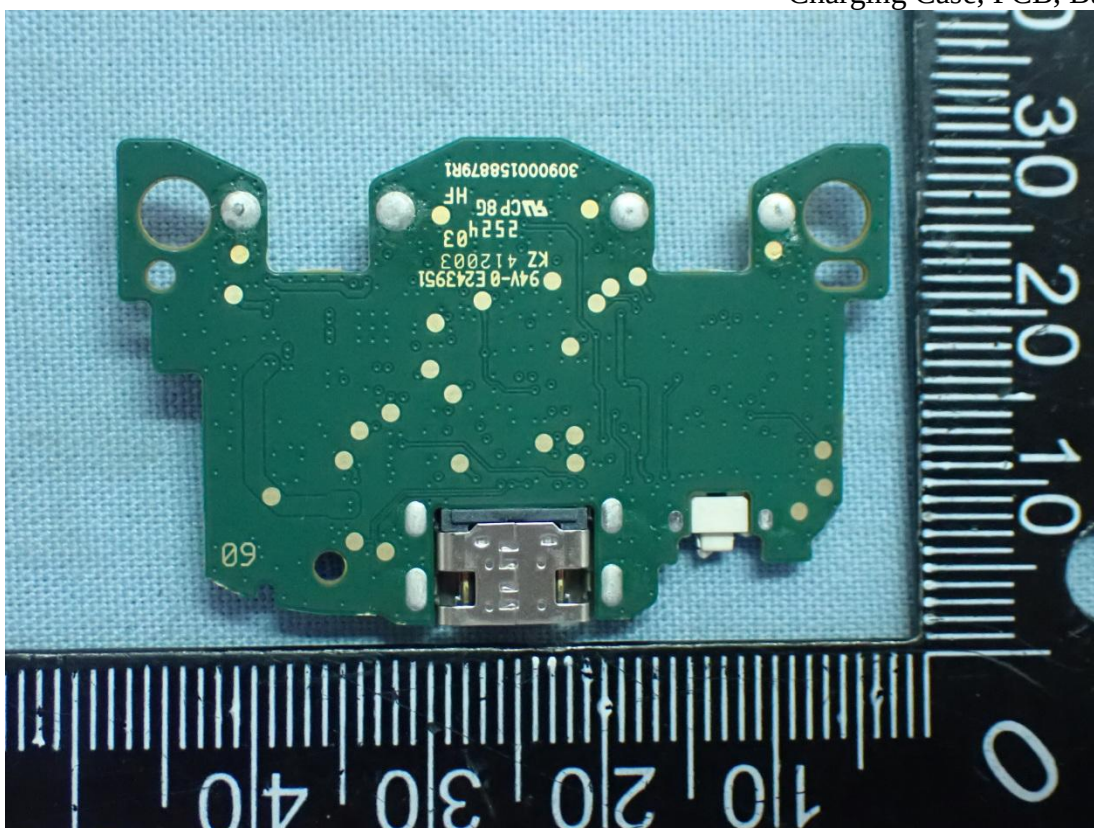
Figure 46 Charging Case, PCB, Back View
