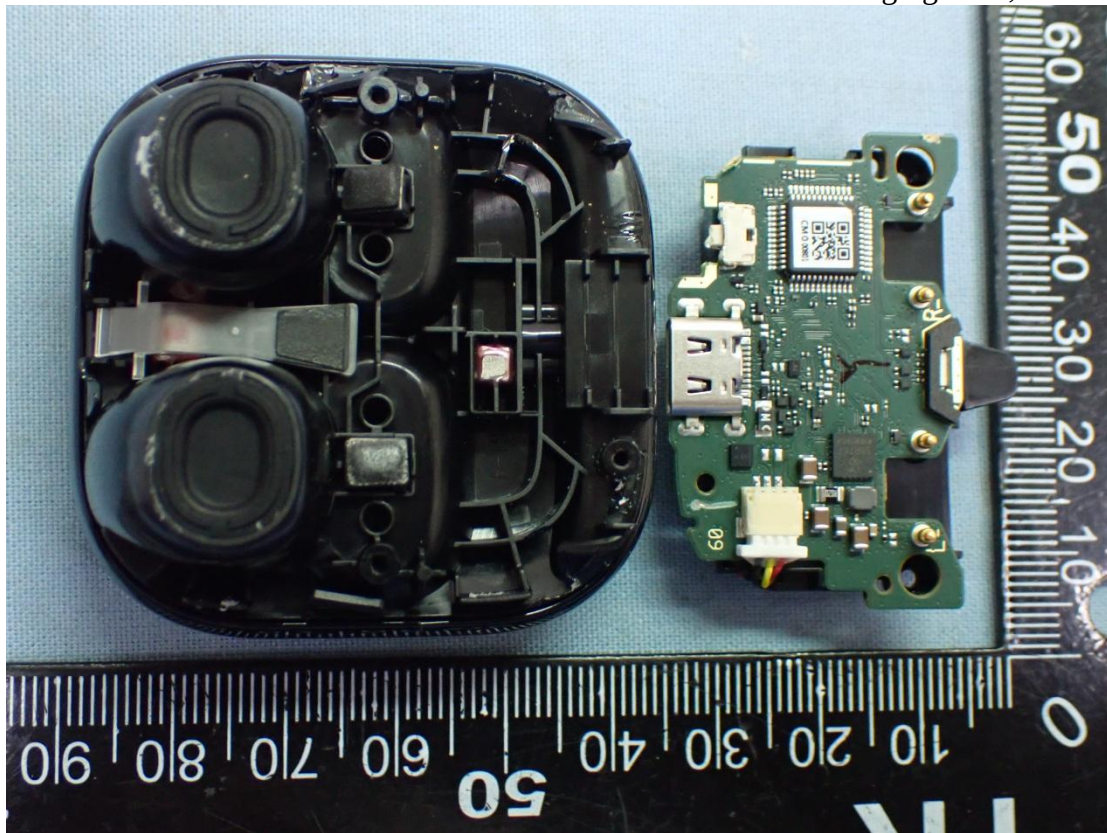
Figure 40 Charging Case, Internal View
