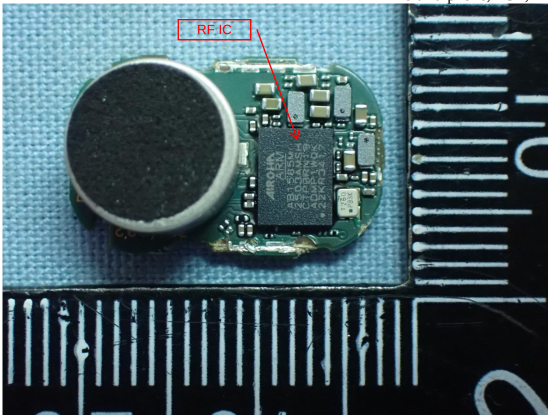
Figure 36 Left Earphone, PCB, Back View
