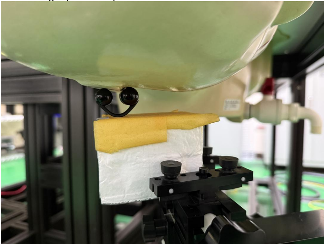
Earbud: Right (Front Side)
