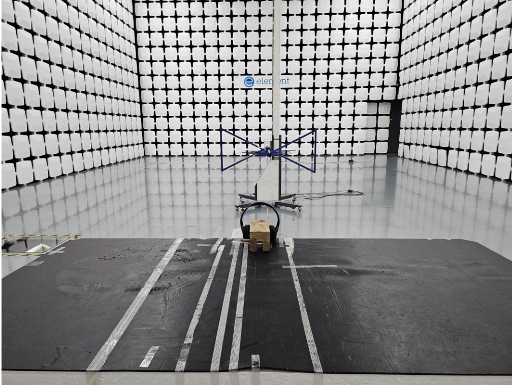
1 GHz Below
