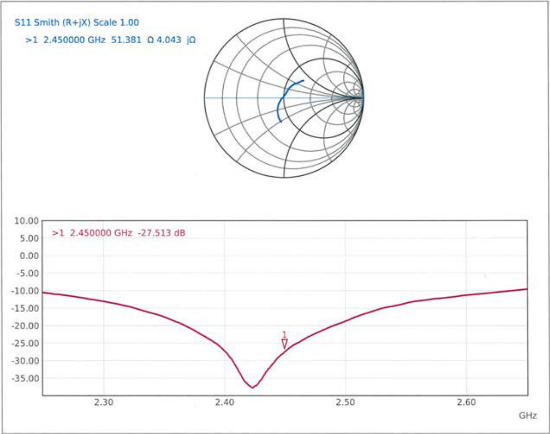
Impedance Measurement Plot for MSL
