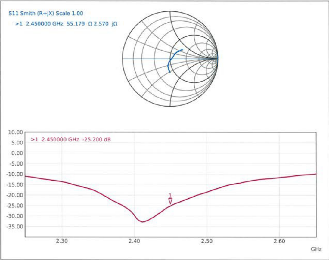
Impedance Measurement Plot for HSL
