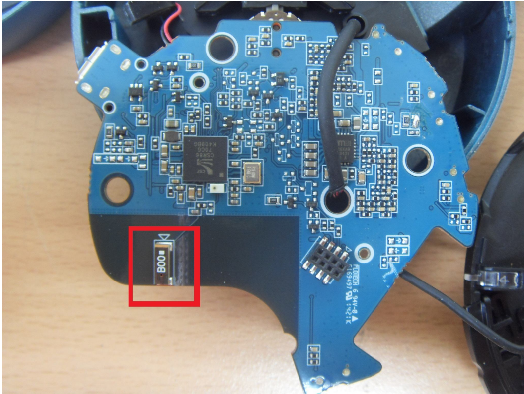
Bluetooth Antenna
