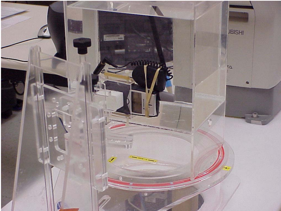
Photo 5: Side view Ericsson phone and EUT both in belt worn position (EUT configuration #1).
