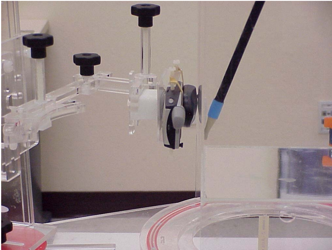
Photo 6: EUT attached to ericsson cell-phone. 1.5cm phone to phantom, EUT touching phantom (EUT configuration #2).
