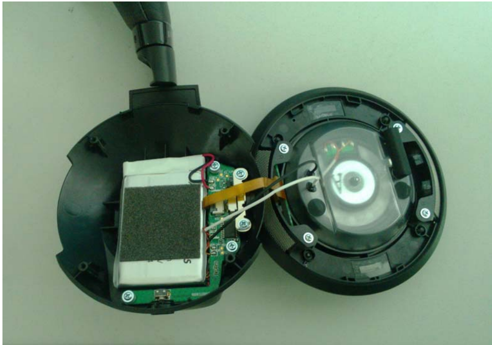
(1) EUT Photo
