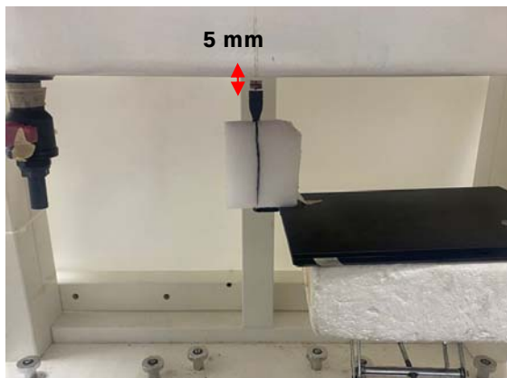
Fig.5 EUT Tip_with cable side to flat phantom
