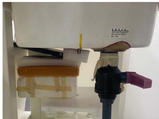
Fig.8 EUT Vertical-Front side to flat phantom
