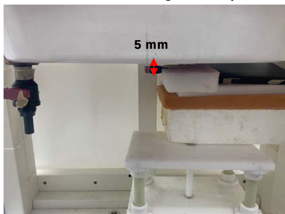
Fig.7 EUT Vertical-Back side to flat phantom
