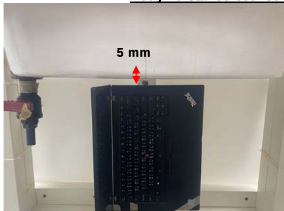
Fig.6 EUT Tip_without cable side to flat phantom
