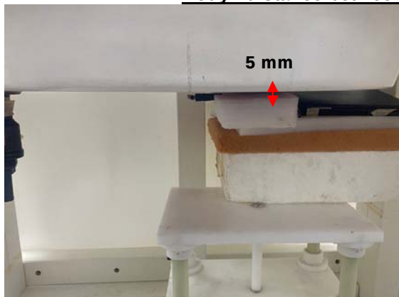
Fig.3 EUT Horizontal-Down side to flat phantom
