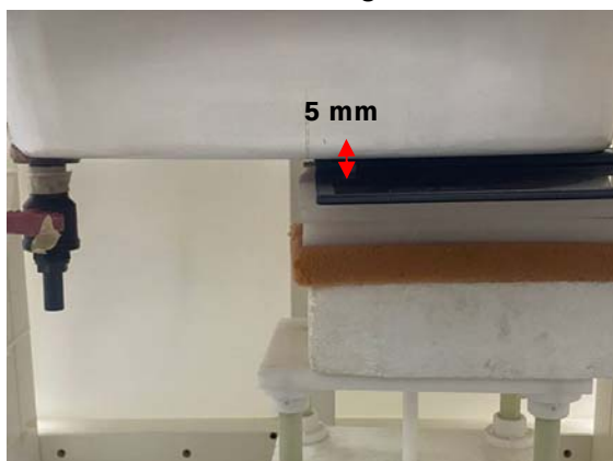
Fig.4 EUT Horizontal-Up side to flat phantom
