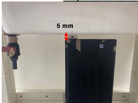
Fig.6 EUT Tip _without cable side to flat phantom
