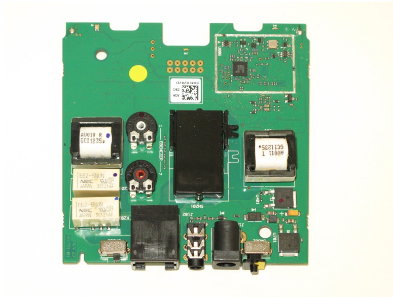
PCBS Bottom –Shield Removed
