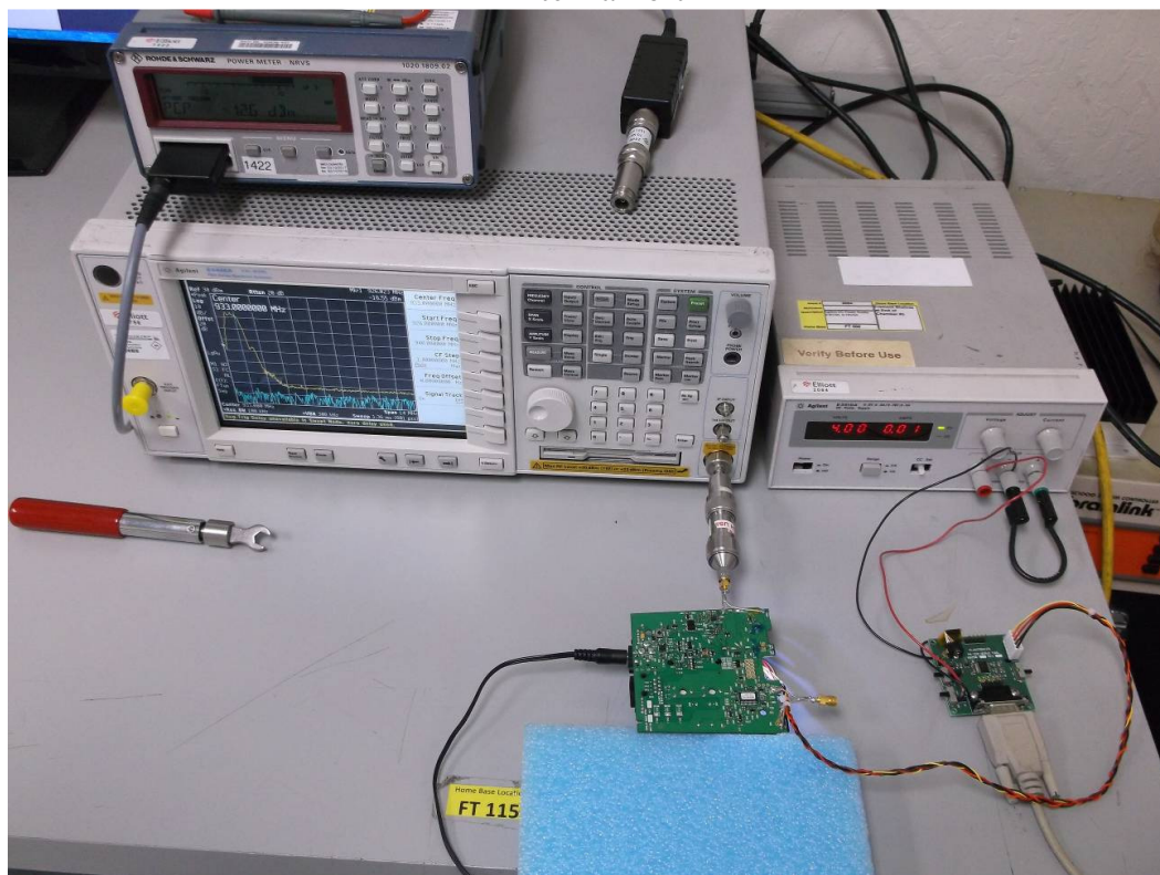
Antenna Port
