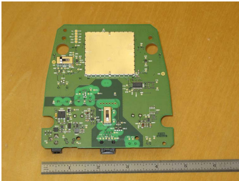
PCB Bottom Shield Installed
