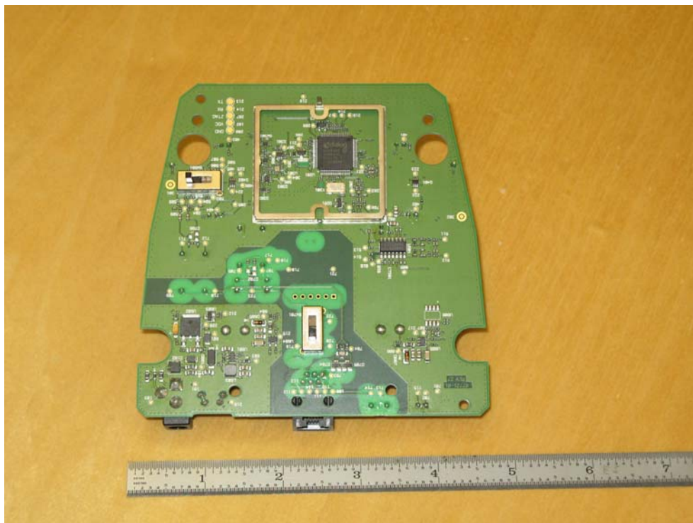
PCB Bottom Shield Removed
