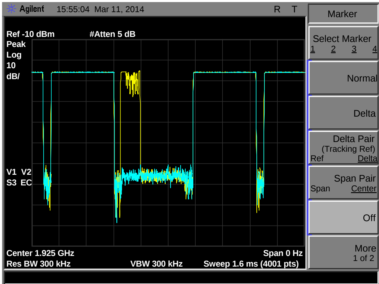
Fig. 68 - Zero-span (single frequency receiver mode) sweep of TDMA interference on carrier at 1924.992MHz, f_i , with base EUT transmission in single open timeslot, detail of open timeslot and transmission.
