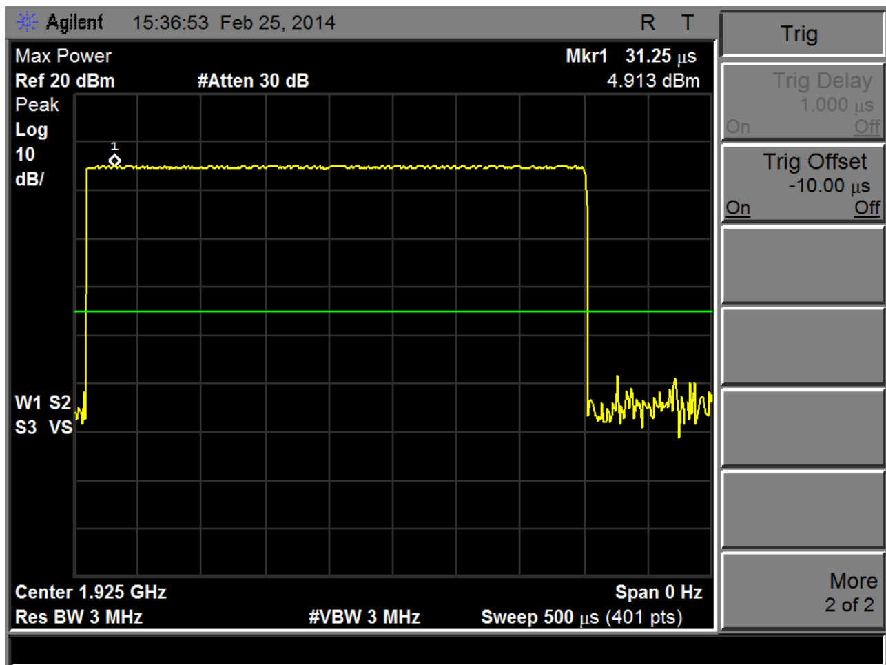
Fig. 11- Base EUT transmit power received by spectrum analyzer configured according to the requirements of clause 6.1.2 of of C63.17-2006, mid carrier. Maximum observed transmit power is 4.91dBm.
