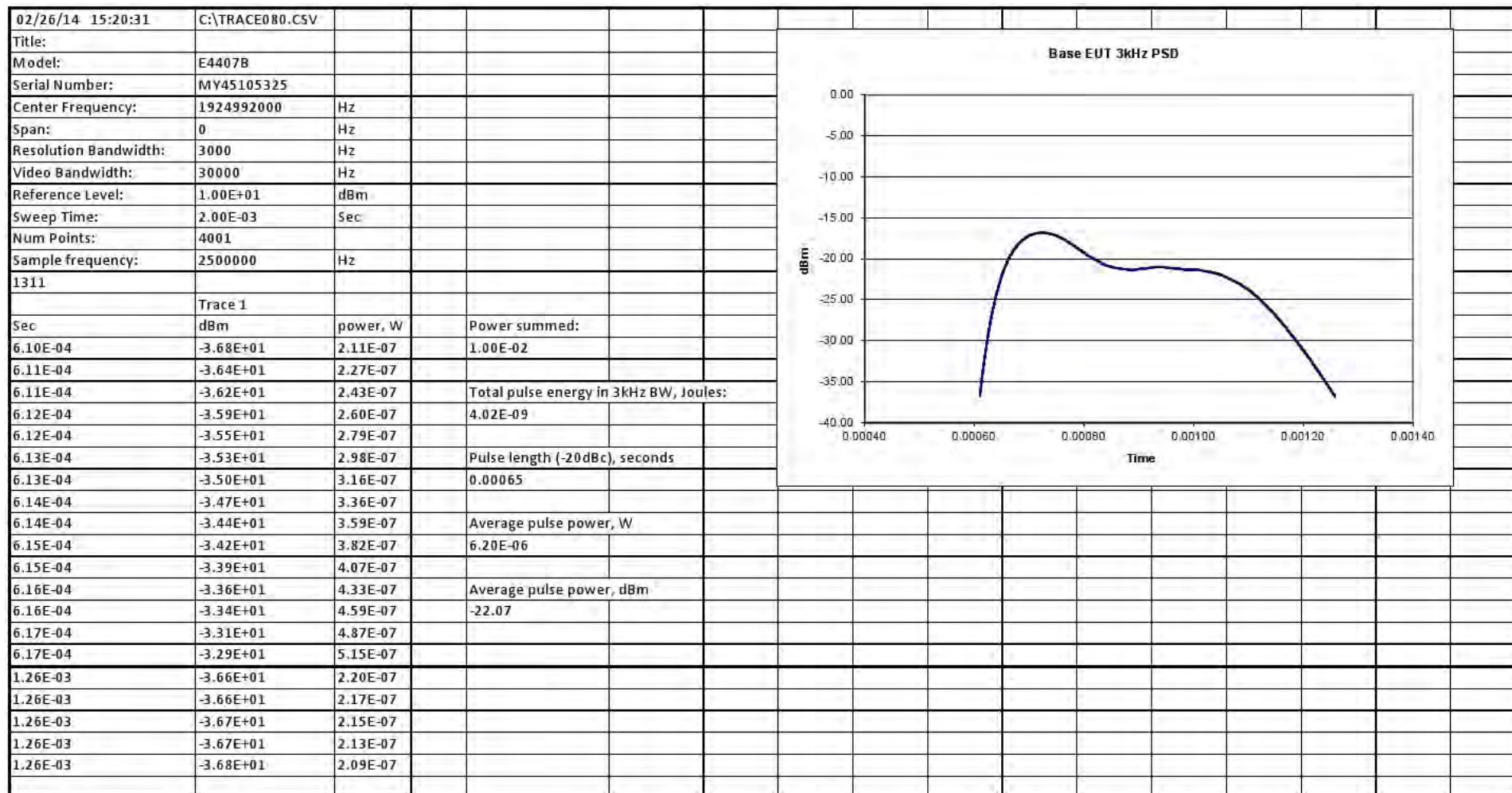
Fig. 19 – Screenshot of Excel file showing PSDlimit calculations for base EUT, mid carrier; -22.07dBm.
