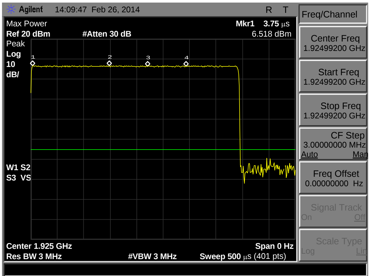
Fig. 81 - Remote EUT transmit power received by spectrum analyzer configured according to the requirements of clause 6.1.2 of C63.17-2006, mid carrier. Maximum observed transmit power is 6.52dBm
