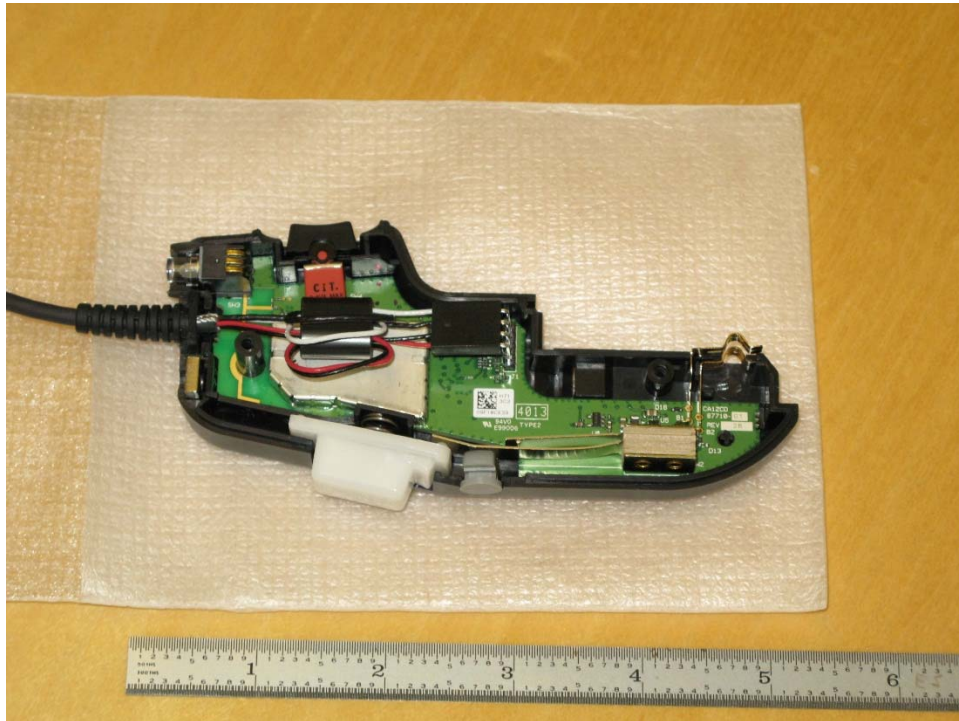
PCB Installed
