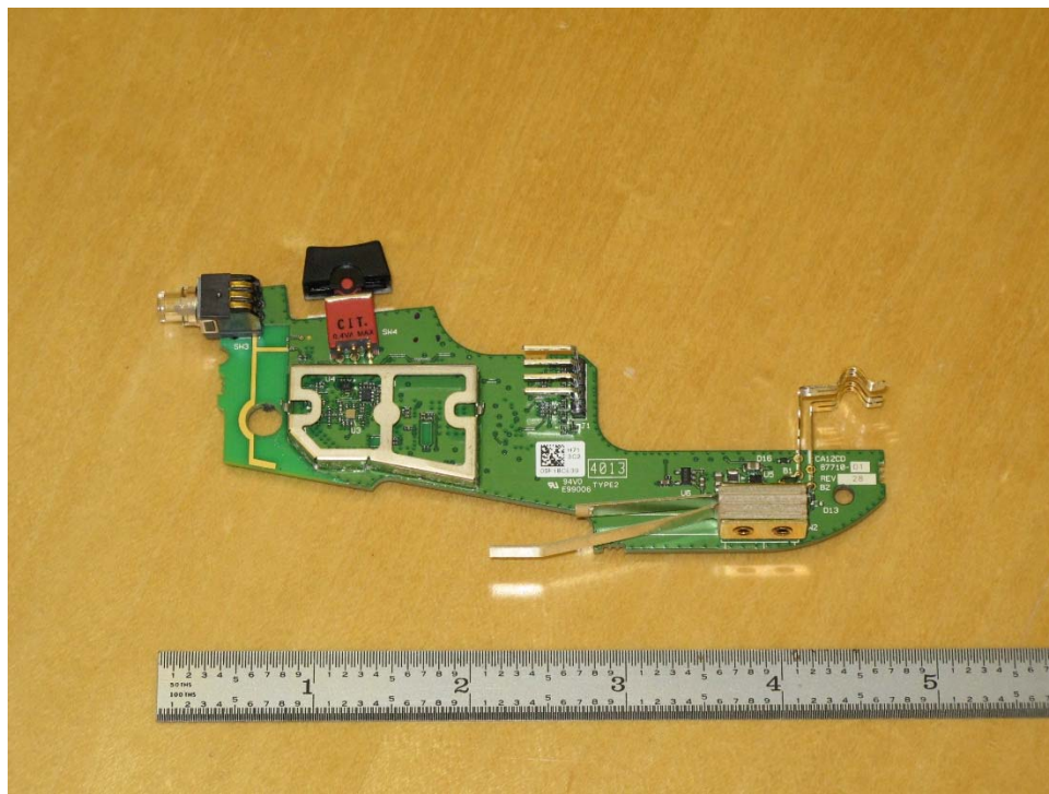
PCB Top Shield removed
