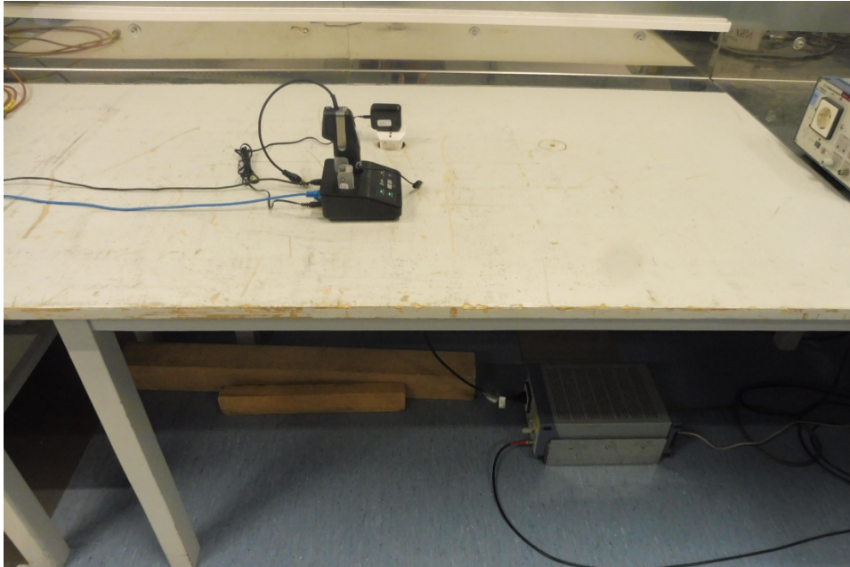
Photo 3: Conducted Emission
