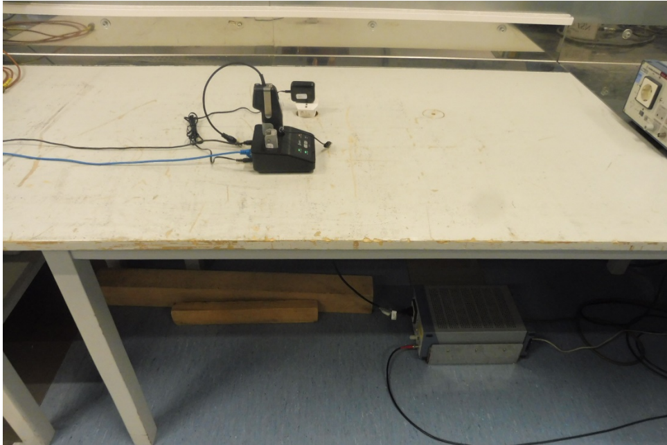
Photo 3: Conducted Emission
