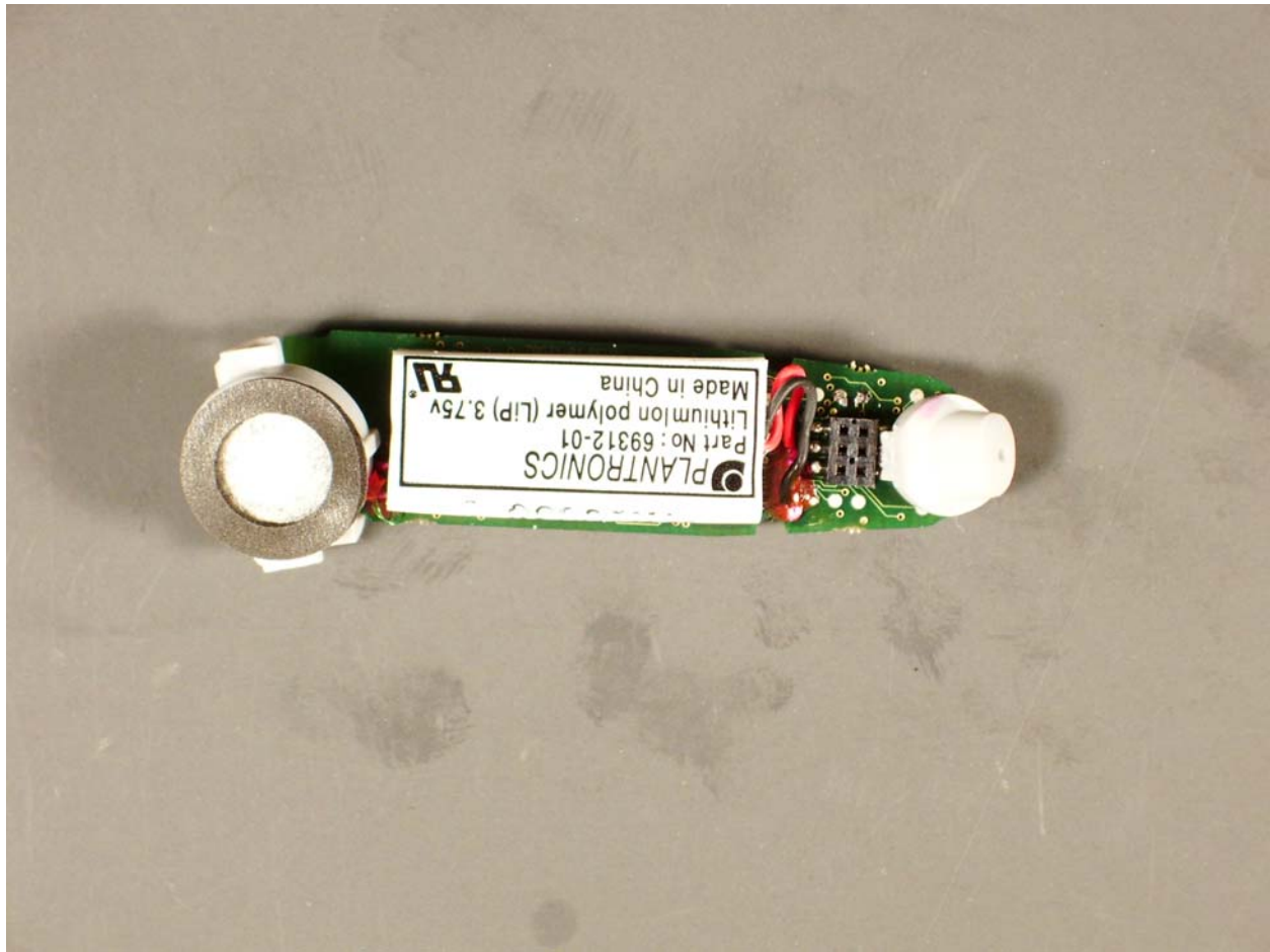
PCB Bottom View – Battery in Place
