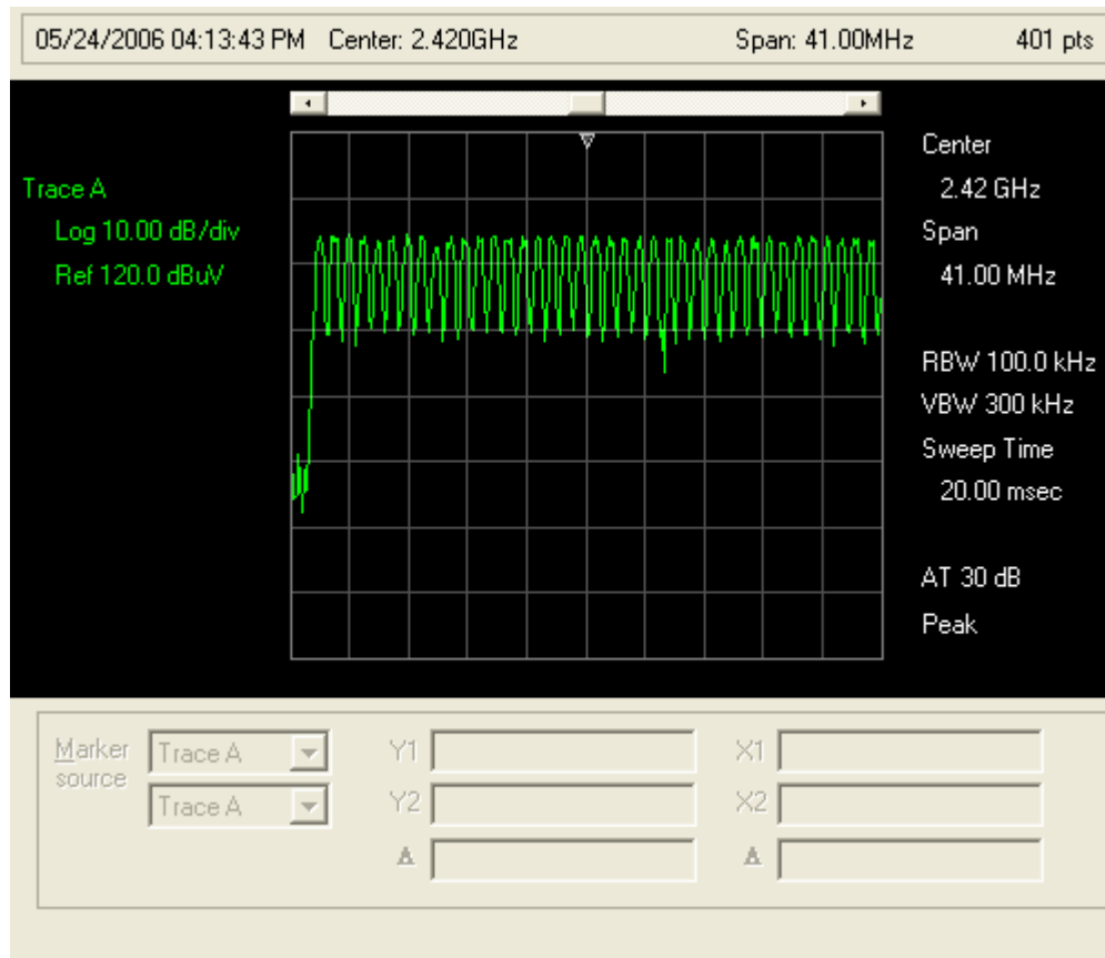
Plot 5: Number of Hopping Frequencies (1)
