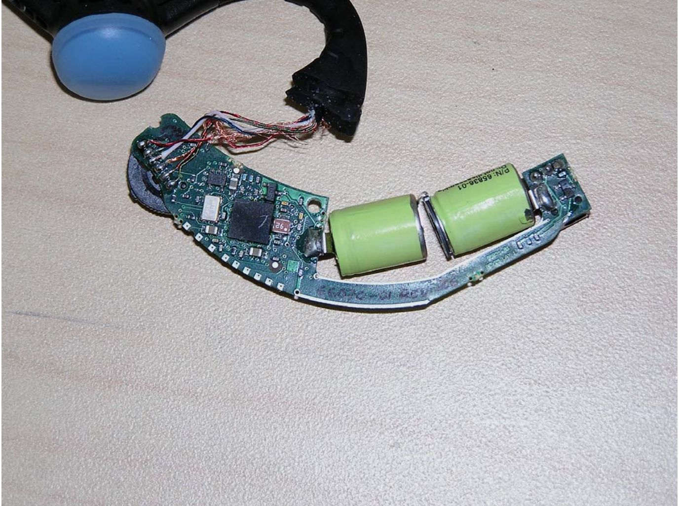
EUT – PCB Top view
