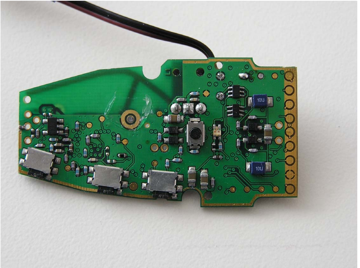
PCB – Bottom view
