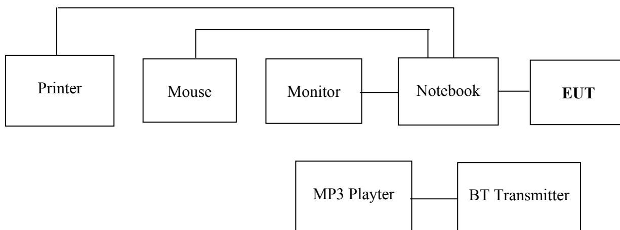
Fig. 2-3 Configuration of Tested System (AC Power Line Conducted Emission/USB Port of PC)
