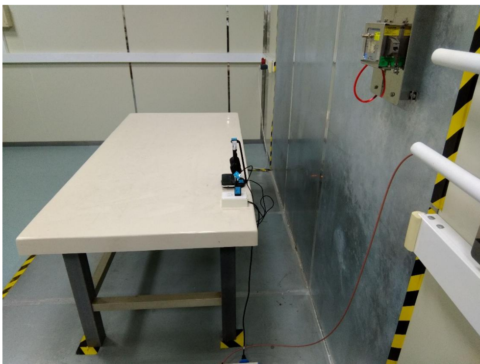
Description: Back View of Conducted Emission Test Setup _Mode 5
