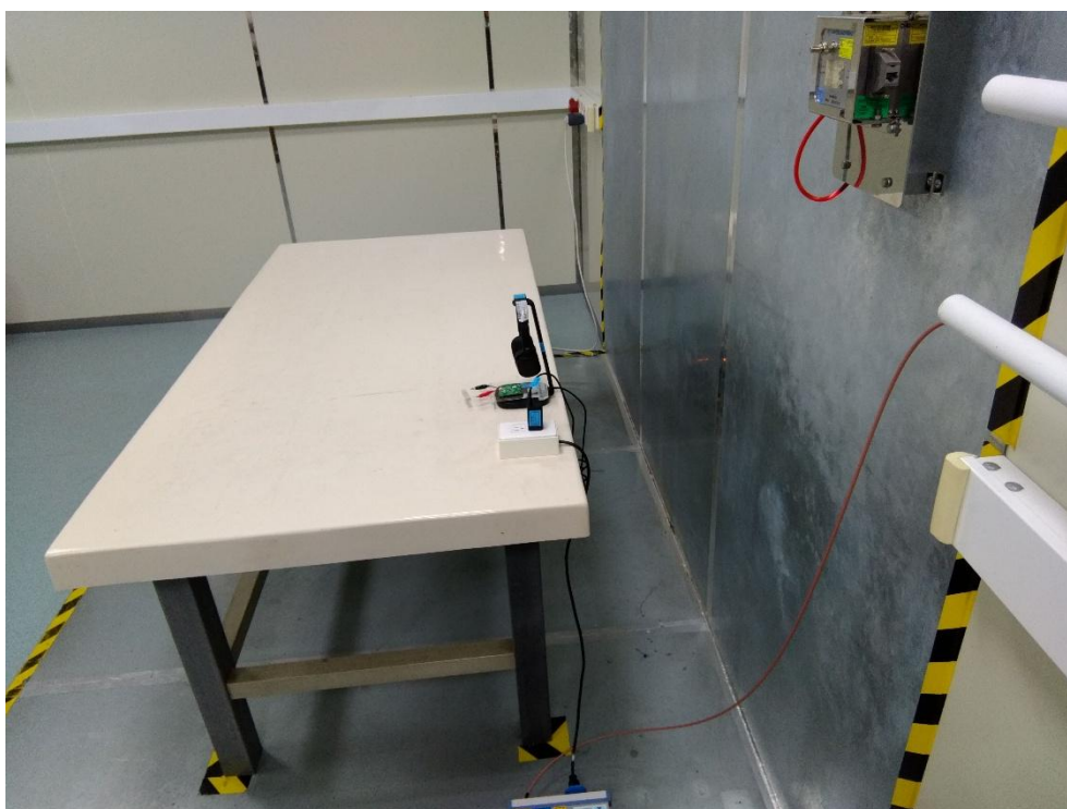
Description: Back View of Conducted Emission Test Setup _Mode 4
