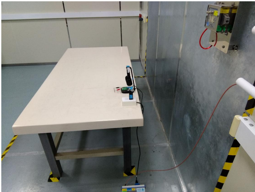
Description: Back View of Conducted Emission Test Setup _Mode 3
