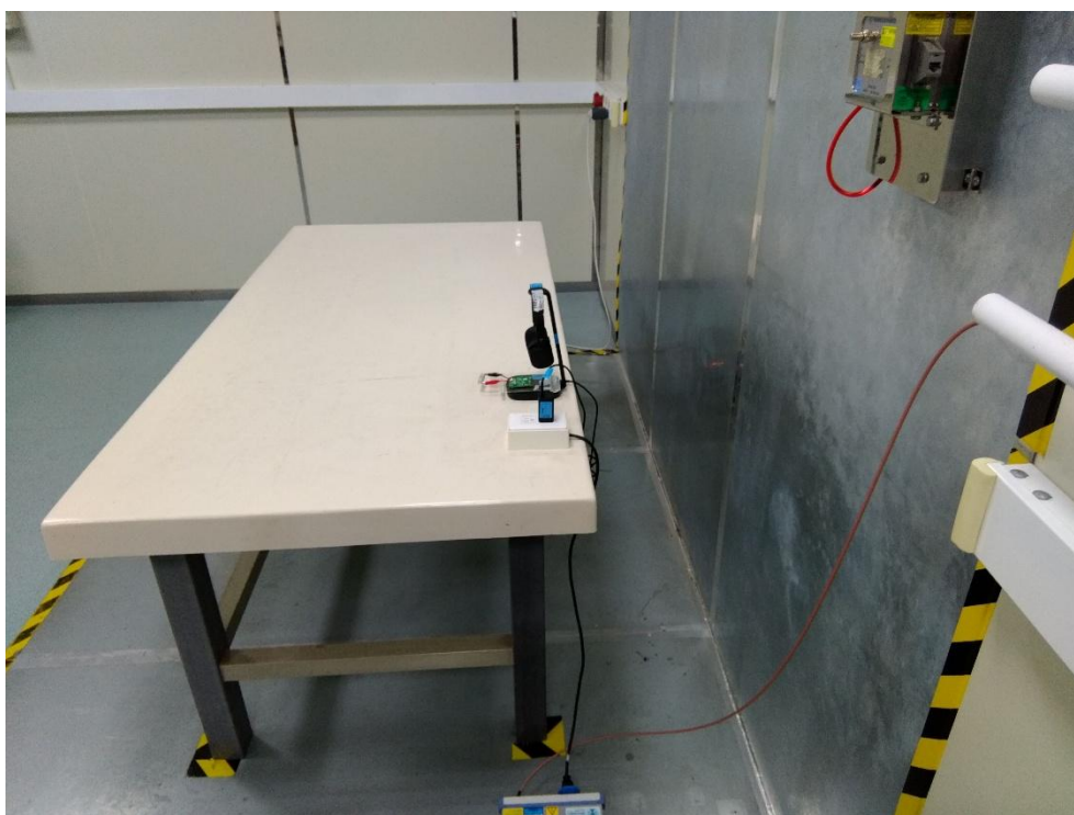
Description: Back View of Conducted Emission Test Setup _Mode 2
