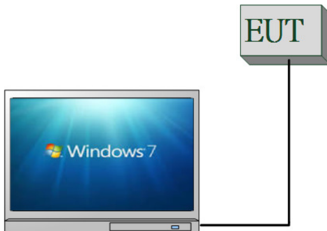
Fig. 2-1 Conducted (Antenna Port) & Radiated Emission Configuration
