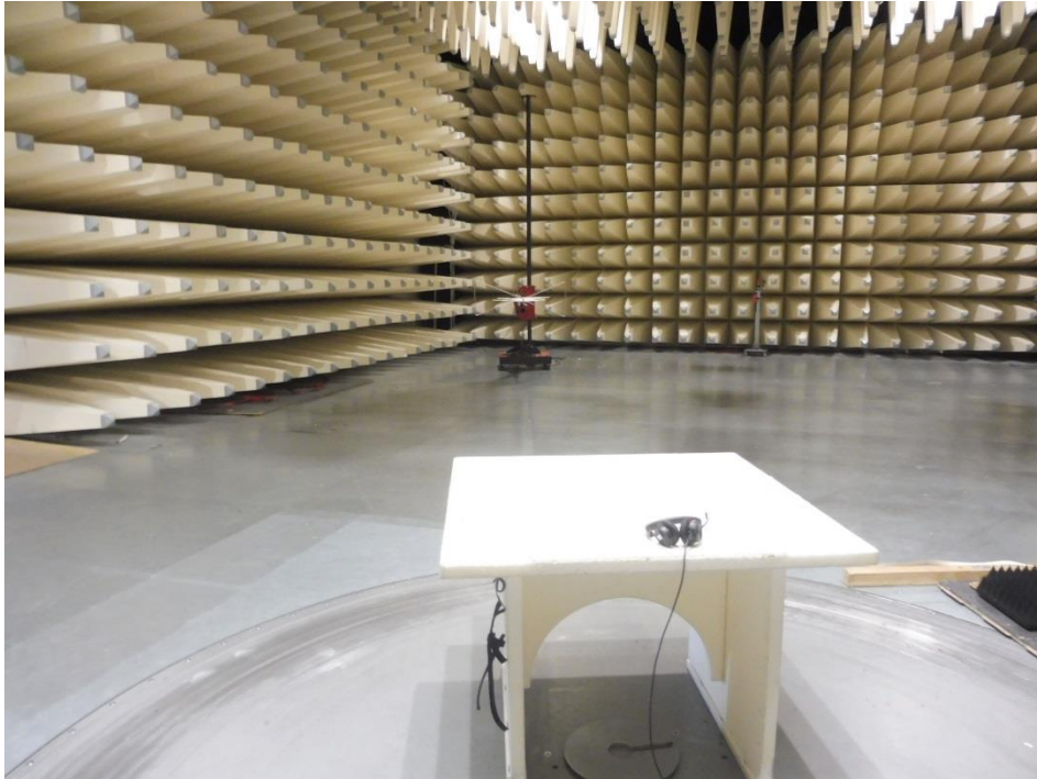
Photo 1: Radiated Emission
