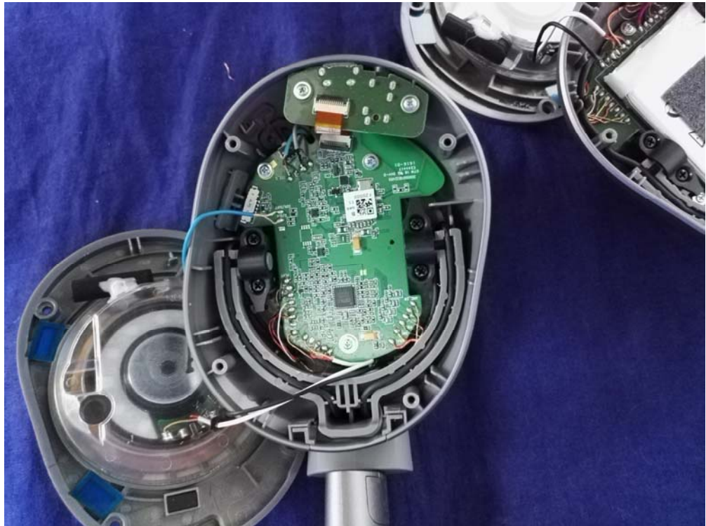
(1) EUT Photo
