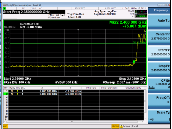
Mode4 (DH5-2)
