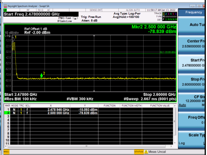
Mode 5 (2DH5-1)
