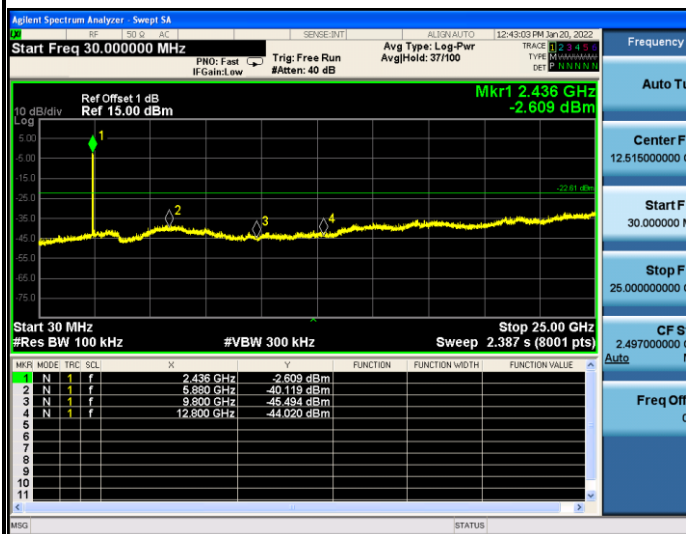
Mode 4 (DH5-2)
