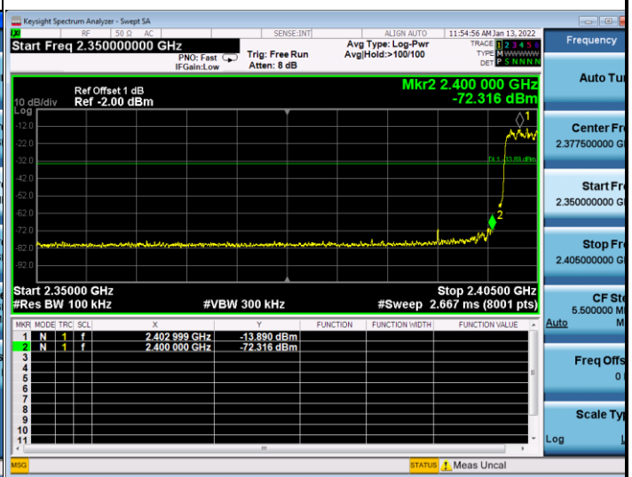
Mode 5 (2DH5-1)
