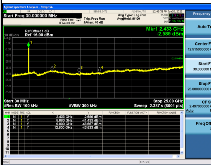
Mode 5 (2DH5-1)
