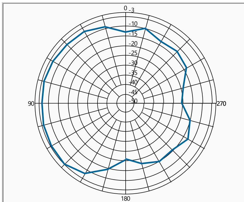
Polar Plot 2
