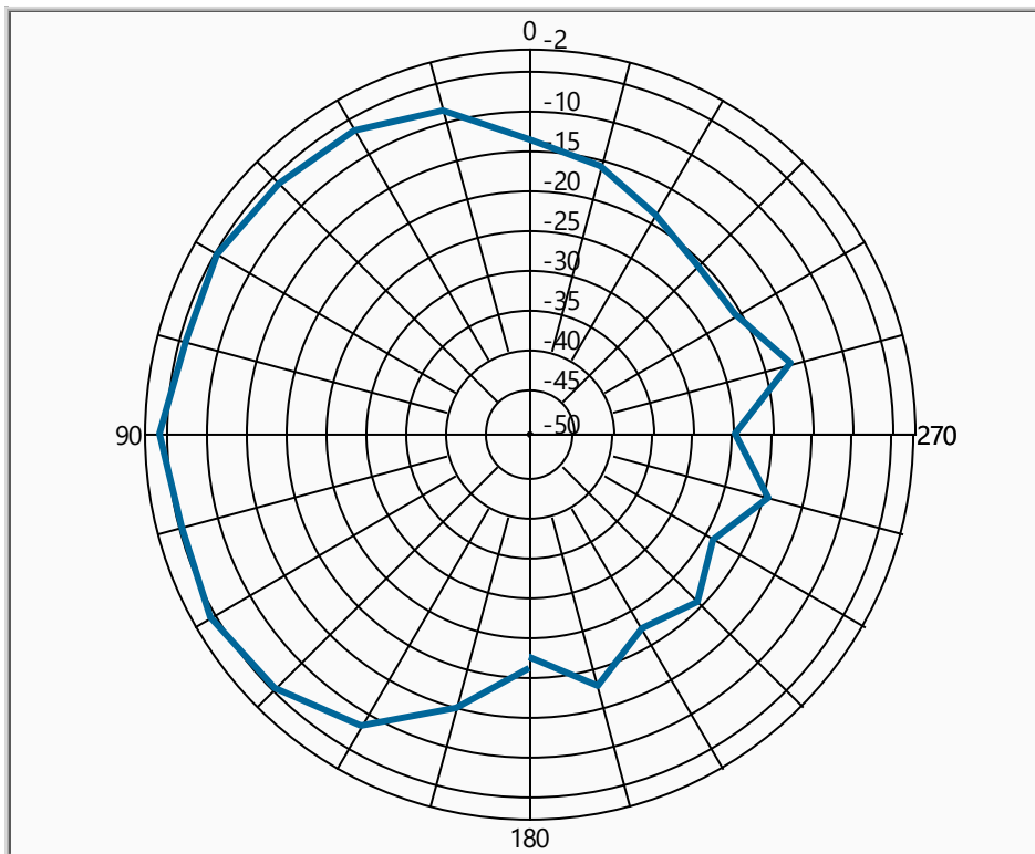
Polar Plot 2
