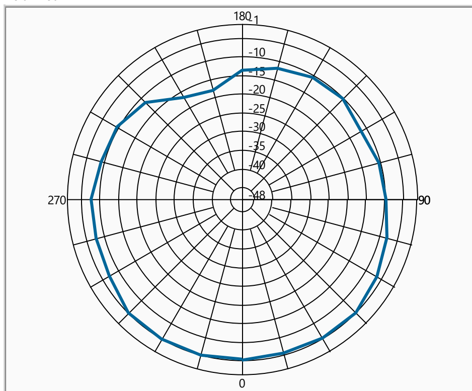
Polar Plot
