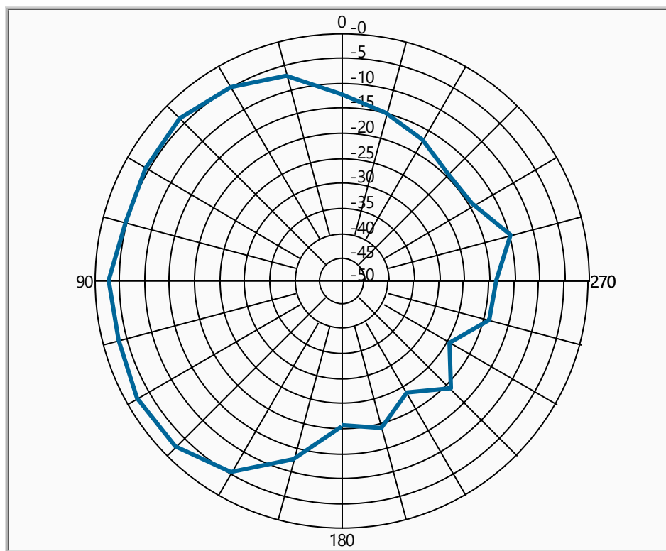
Polar Plot 2
