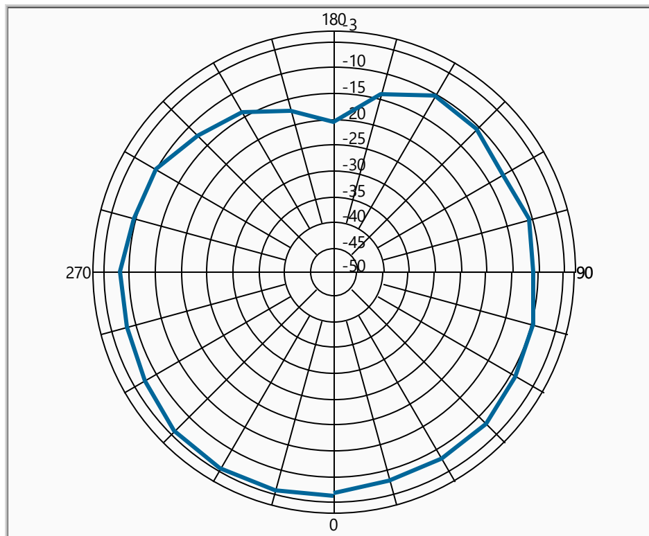
Polar Plot
