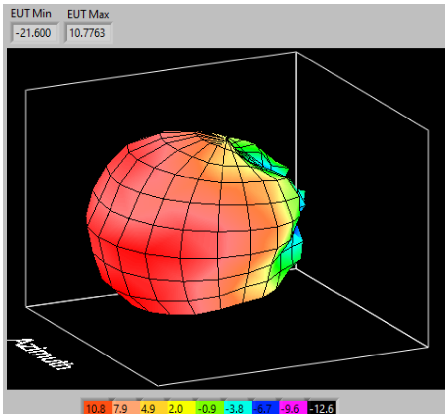
EUT Serial # 0001JA Channel 39 (2441 MHz) Max power 11.78 dBm
