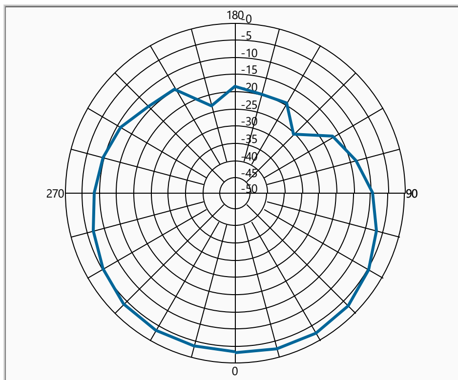
Polar Plot
