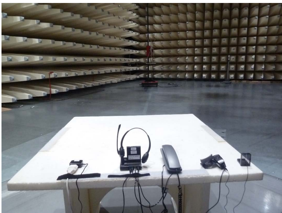
Photo 2: Radiated Emission
