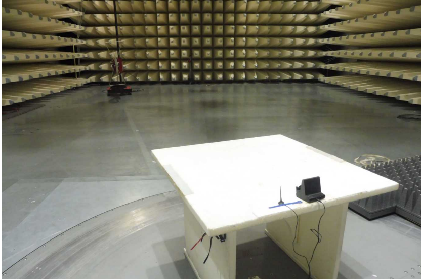
Photo 7: EUT at the semi-anechoic chamber
