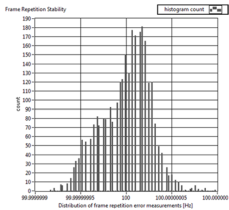
Histogram of Frame Repetition Stability
