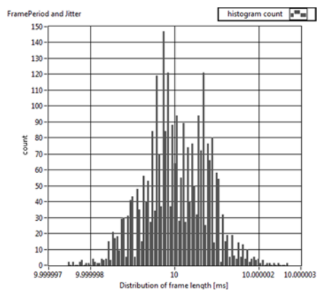
Histogram of Frame Period and Jitter
