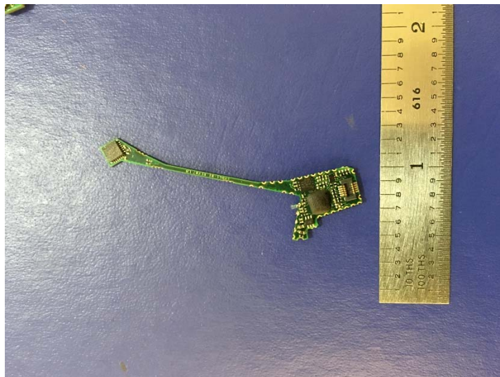
Daughterboard Bottom
