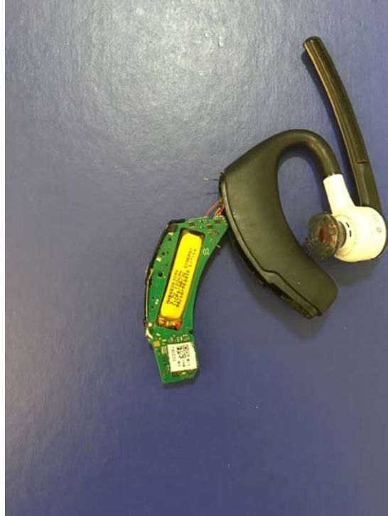
PCBA installed
