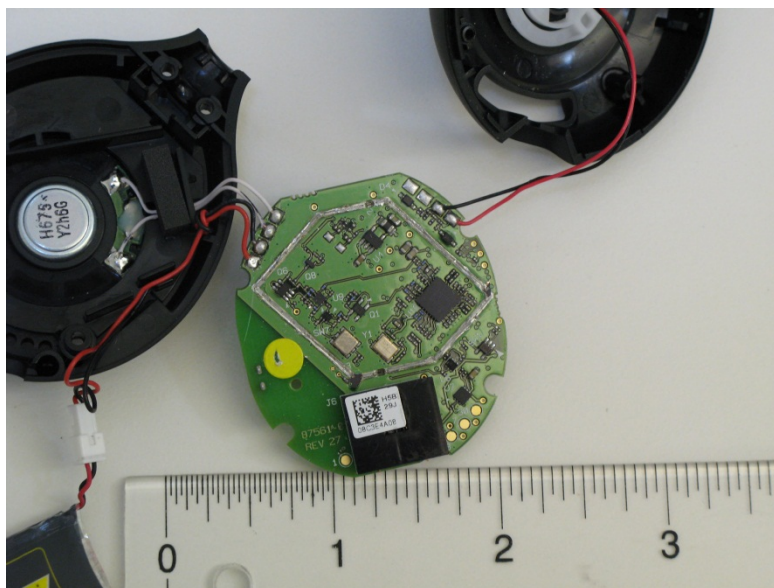
PCBA Bottom Shield removed
