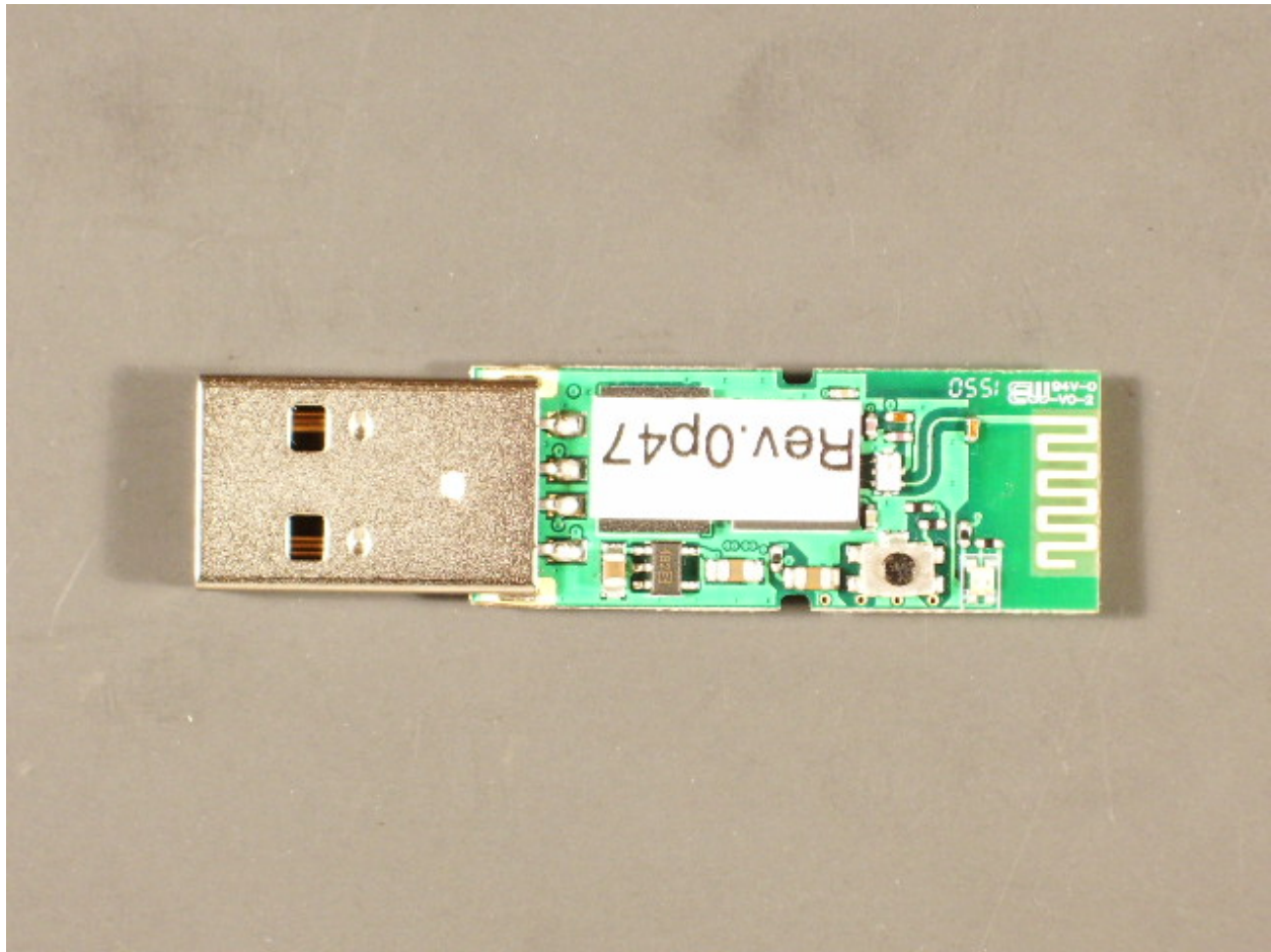
PCB Top View [Antenna Trace to the Right in Photo]
