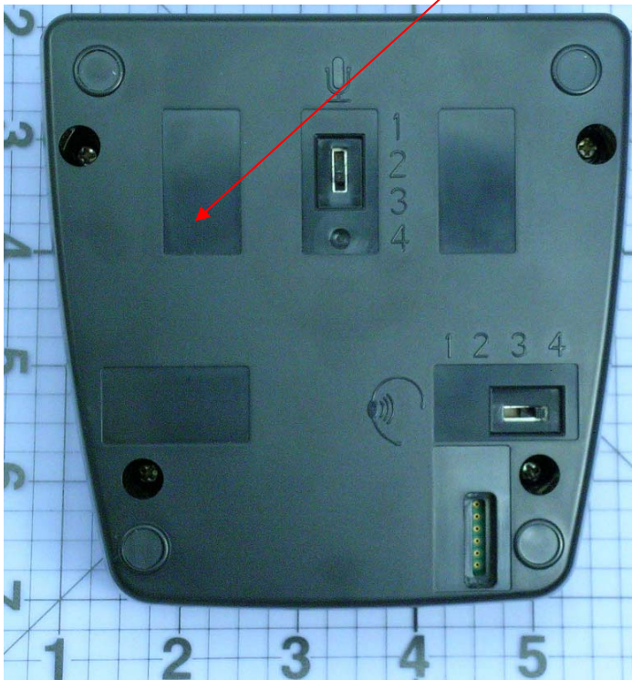
Bottom view
