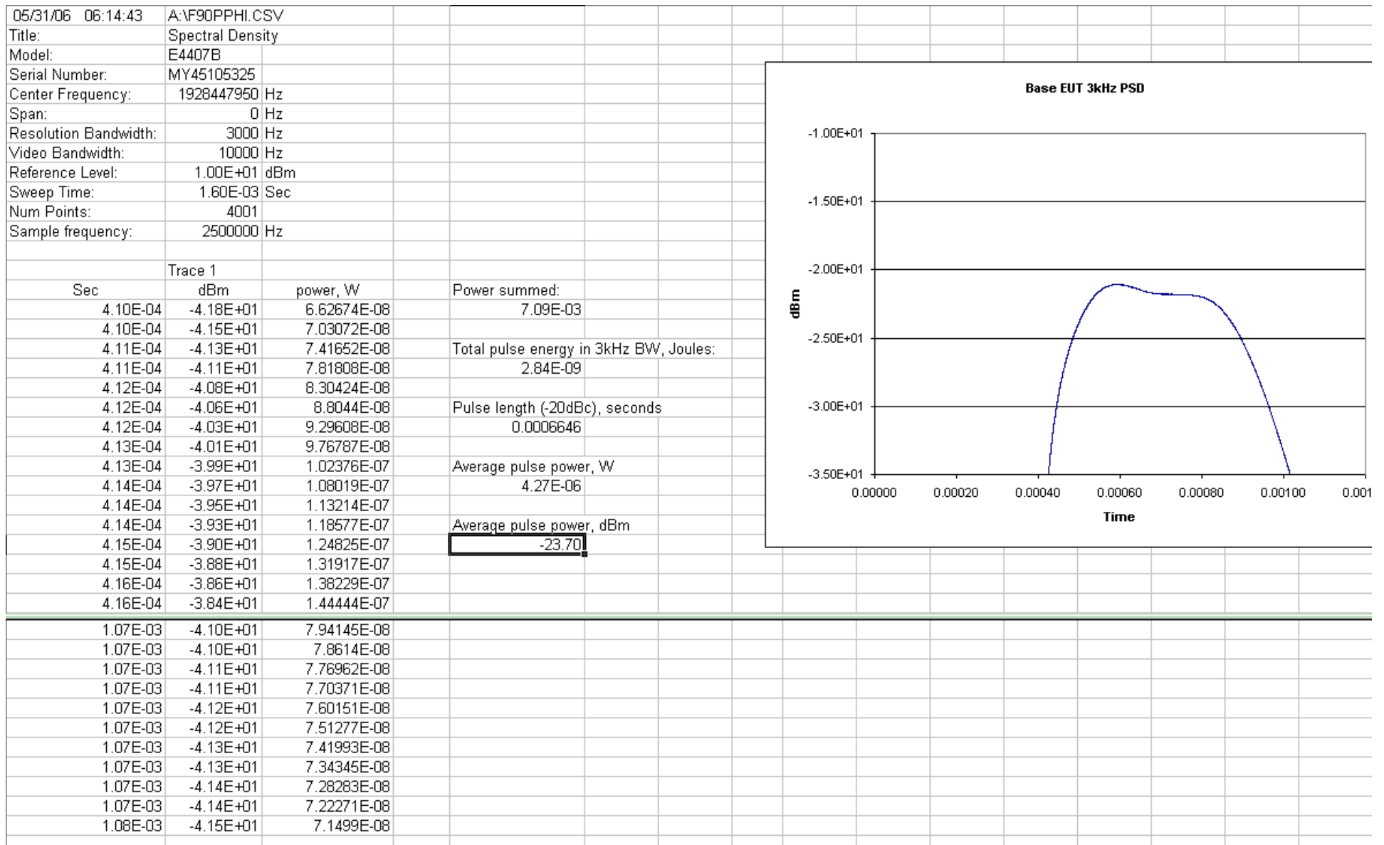
Fig. 91 – Screenshot of Excel file showing PSDlimit calculations for remote EUT, high carrier; -23.70dBm.
