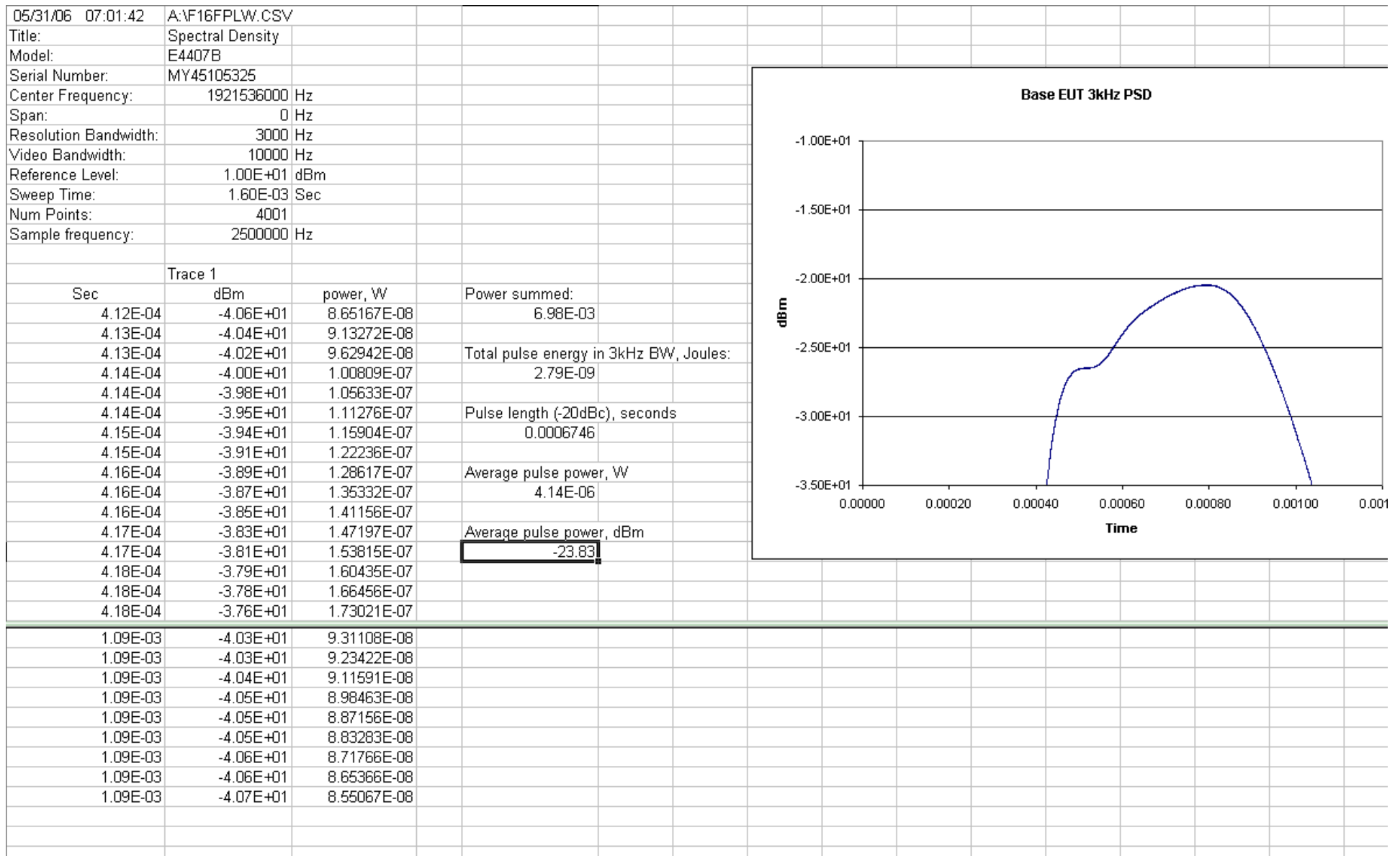
Fig 17 – Screenshot of Excel file showing PSDlimit calculations for base EUT, low carrier; -23.83dBm.
