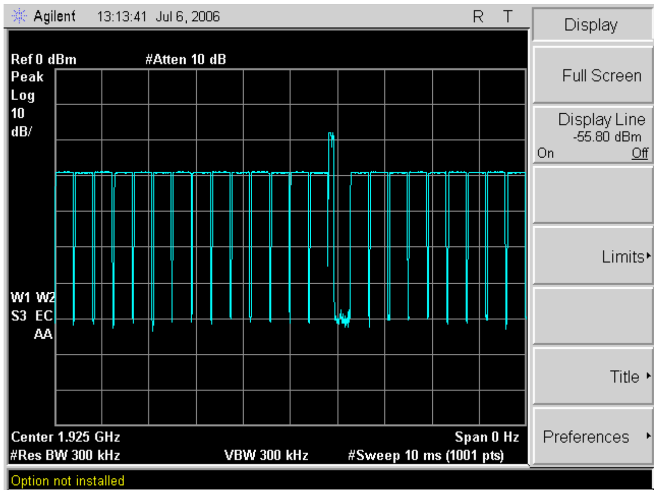
Fig. 70 - Zero-span (single frequency receiver mode) sweep of TDMA interference on carrier at 1924.992MHz, f_i , with base EUT transmission in single open timeslot.
