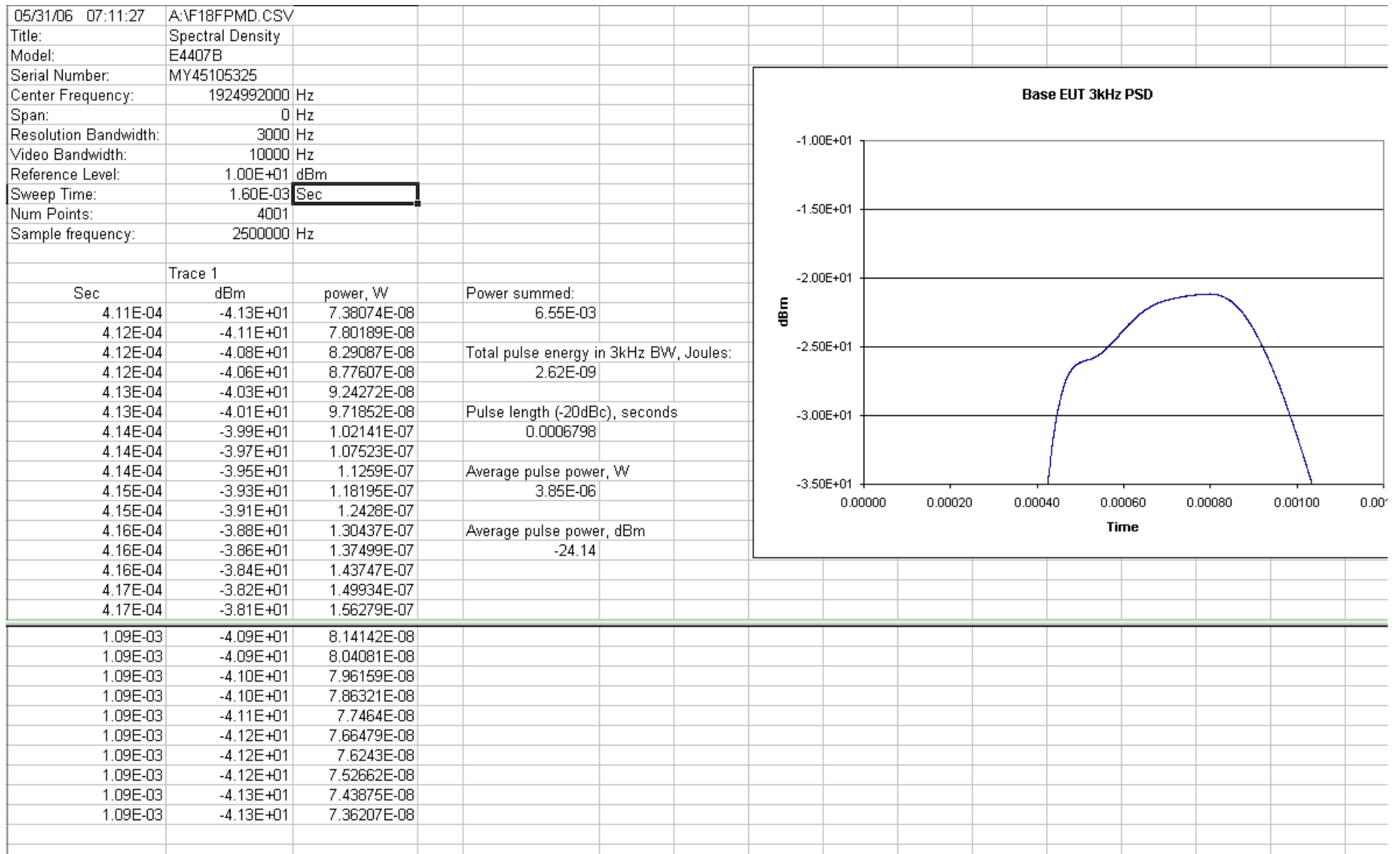
Fig 19 – Screenshot of Excel file showing PSDlimit calculations for base EUT, mid carrier; -24.14dBm.
