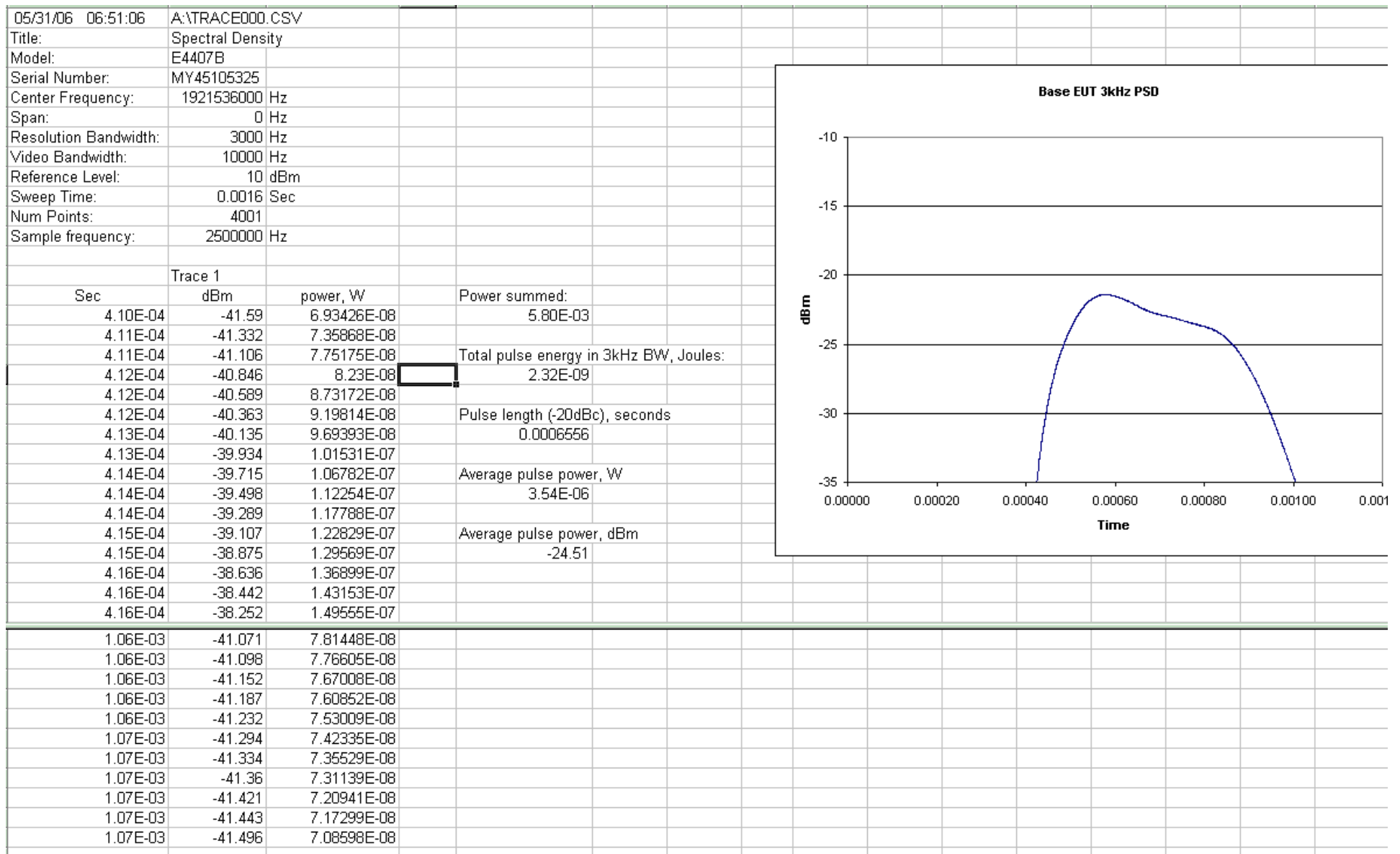
Fig 87 – Screenshot of Excel file showing PSDlimit calculations for remote EUT, low carrier; -24.51dBm.
