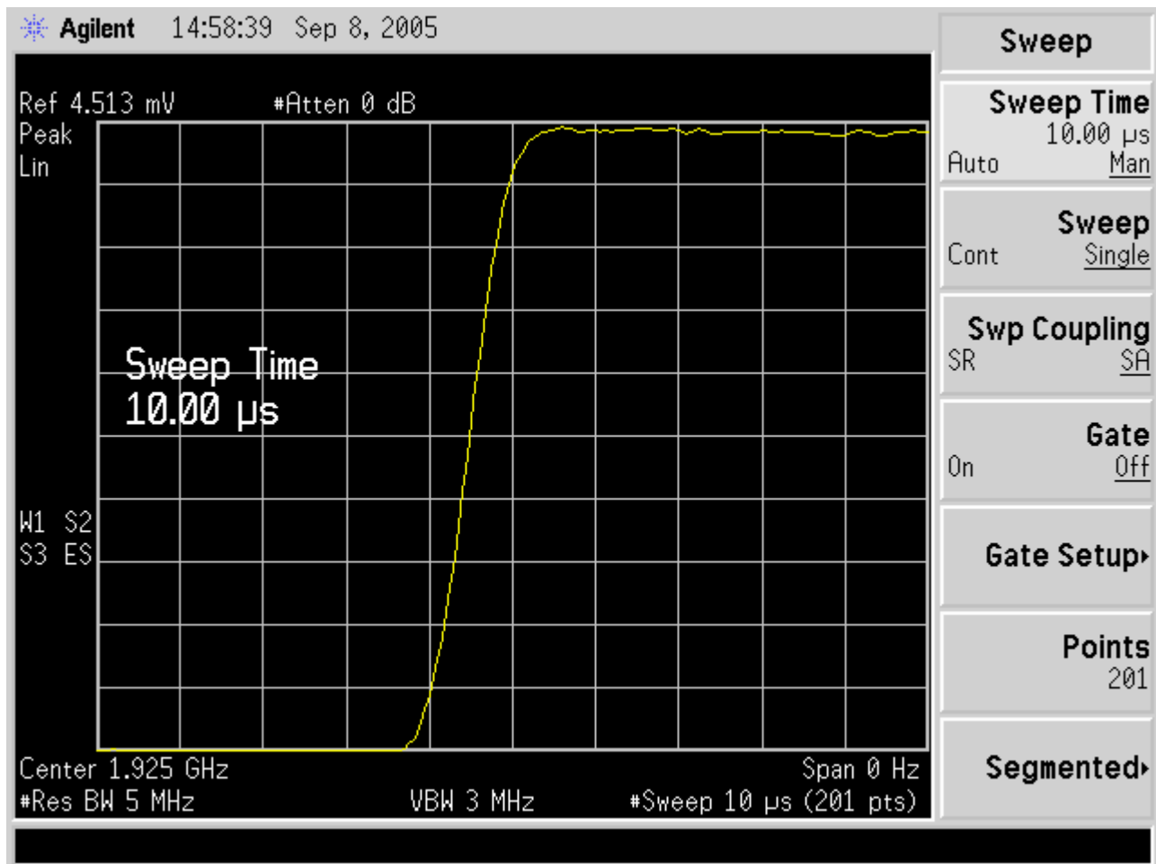
Fig. 62 - Rise time of interference pulse, per the requirements of 7.5 for less than 1uS for 10% to 90% transition.
