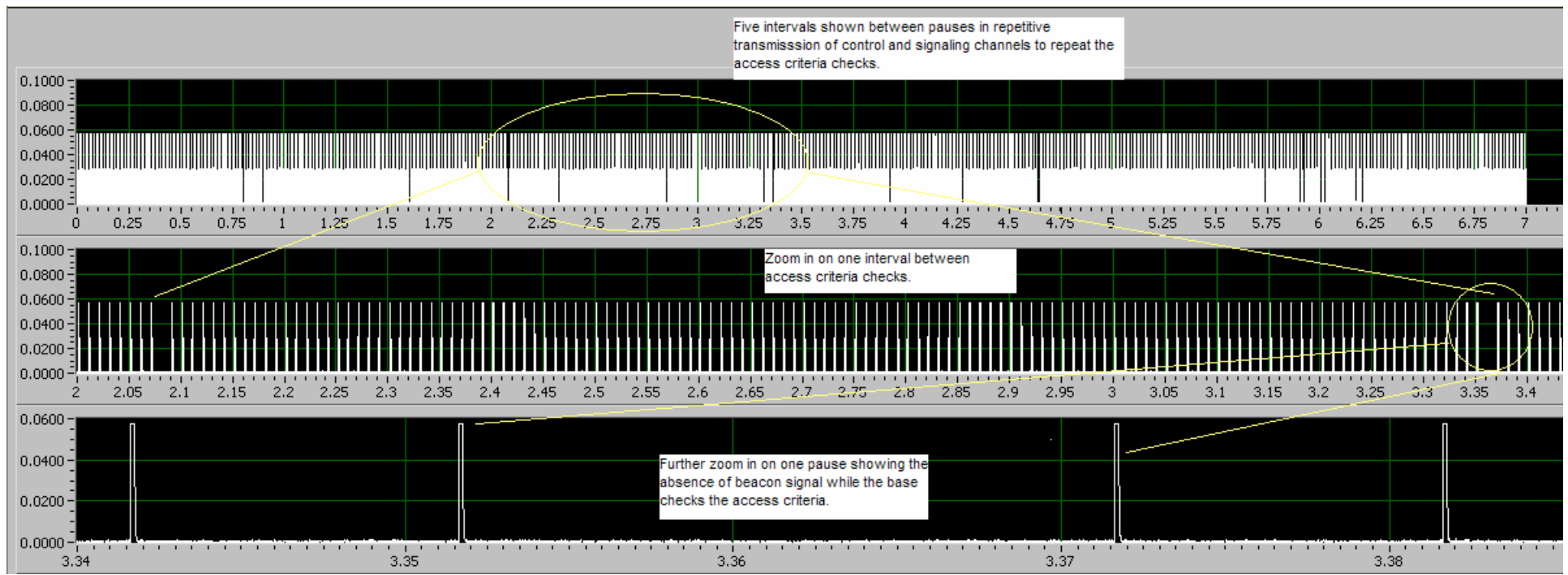
Fig. 72 - Capture of demodulated transmissions of base EUT control and signaling transmissions; the signal present at the RF detector output. The resolution of detail may require viewing this document in electronic format at 150% resolution. Irreducible image artifacts occur in the top trace due to pixilation in the original screen-capture.
