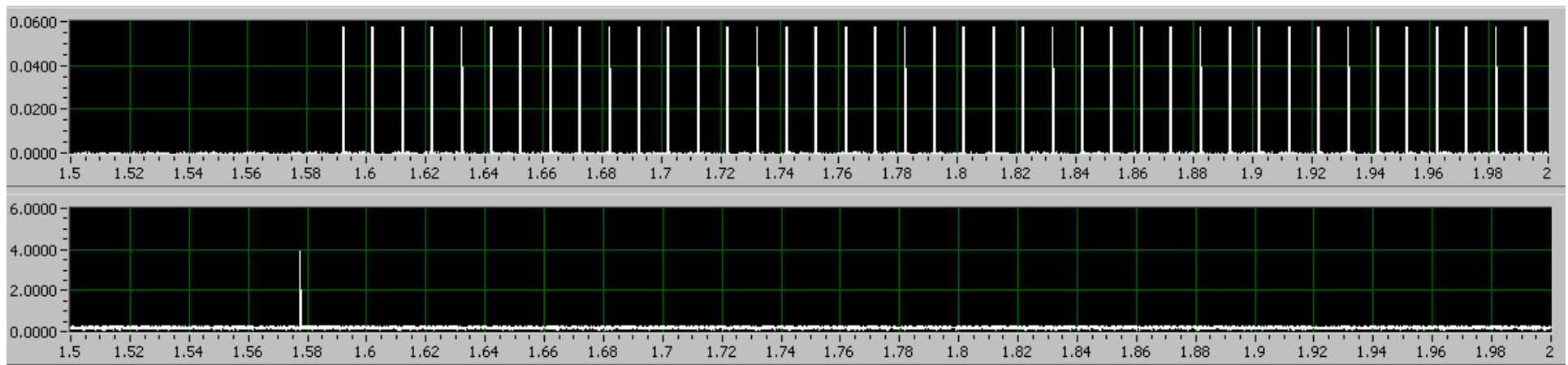
Fig. 127 - Normal initiation of transmissions by the remote EUT in the absence of over-threshold interference; the remote EUT software flags the start of the transmission setup (bottom trace) at t = 1.5658 seconds, and transmit emissions are recovered by the RF detector (top trace) in the splitter/combiner network beginning at t = 1.586 seconds. Proper transmission at T_U - U_M is shown, to validate functionality and to illustrate the getting-ready-to-transmit marker, and the RF detector output.
