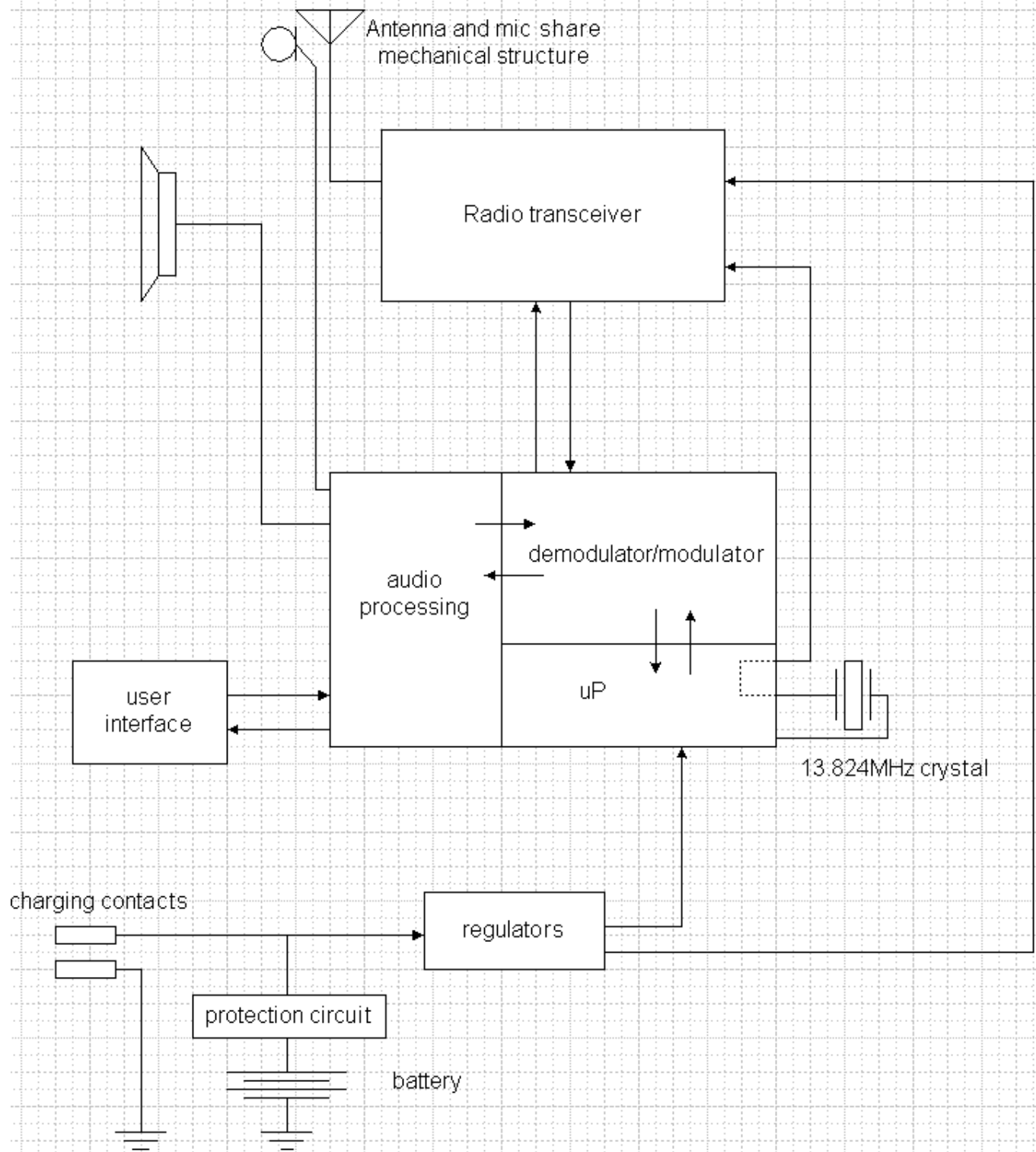
Block diagram of CS50 headset unit
