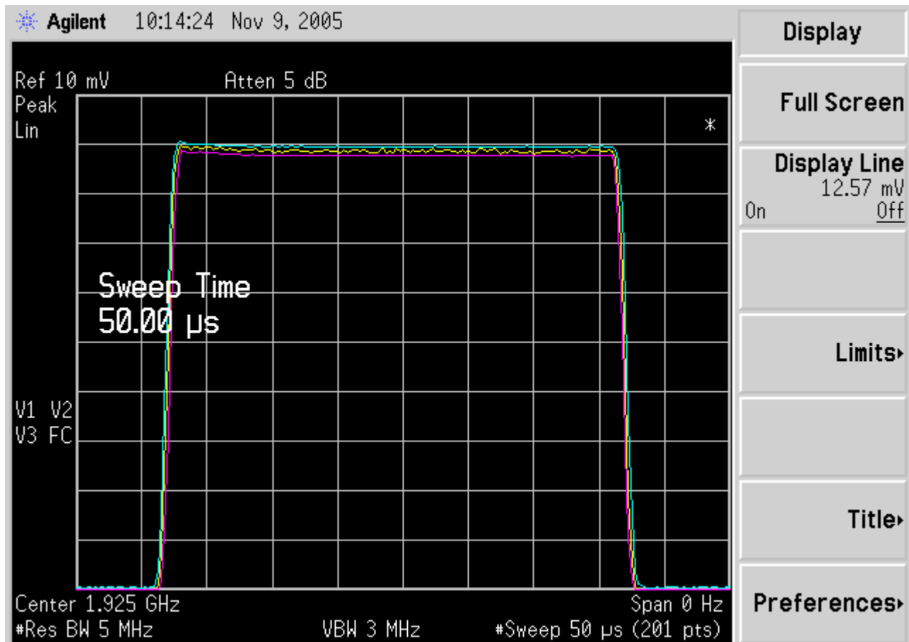
Fig. 59 - 35uS interference pulse for 7.5(d), duration and amplitude variation over the duration of the pulse and over multiple pulses. Spectrum analyzer is set to linear response.
