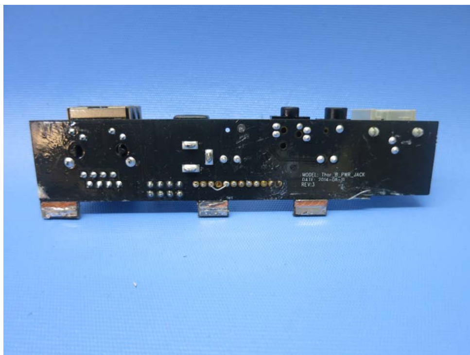
Base Unit Switch PCB solder side
