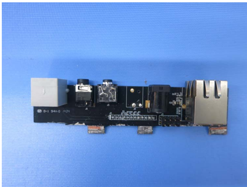
Base Unit Switch PCB comp side
