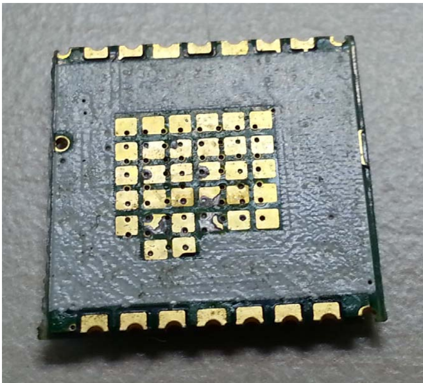
Base Unit WiFi Module solder side
