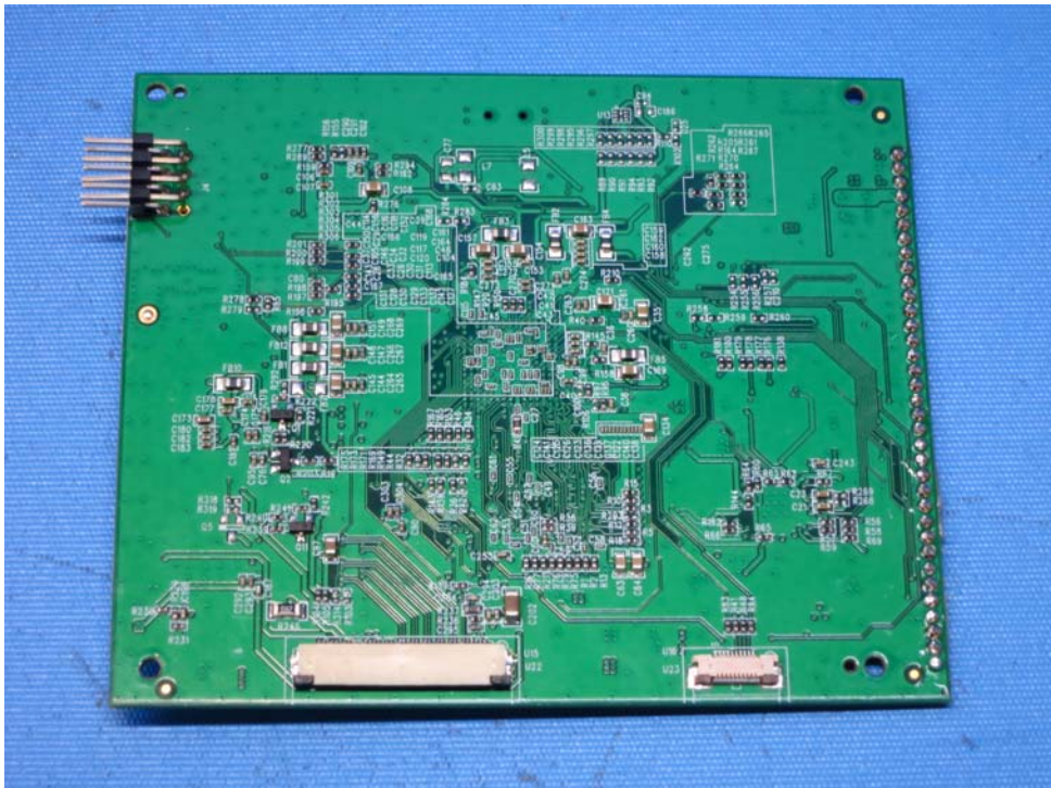
Base Unit AM3354BZCZ100 PCB solder side
