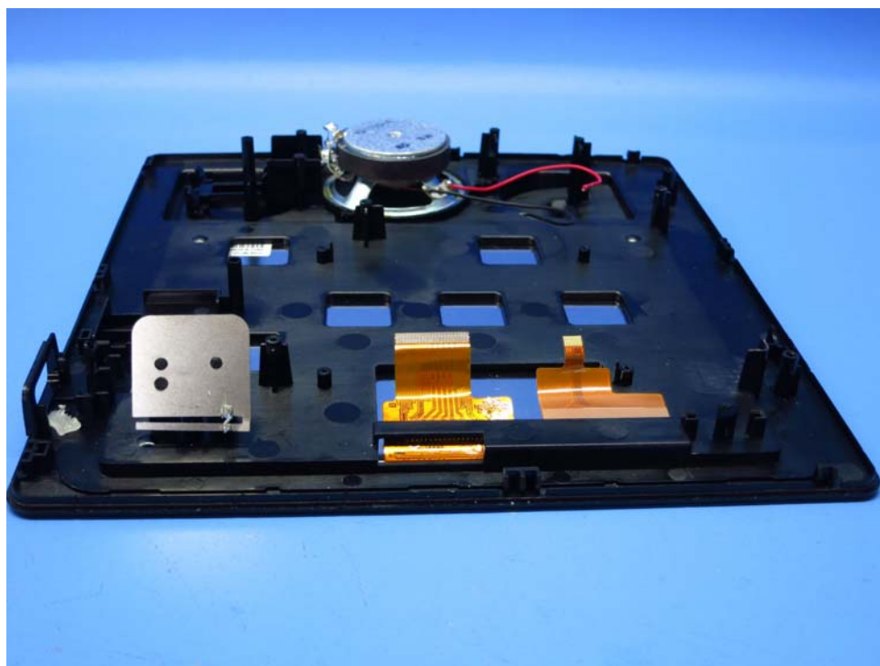
Base Unit – WiFi Antenna
