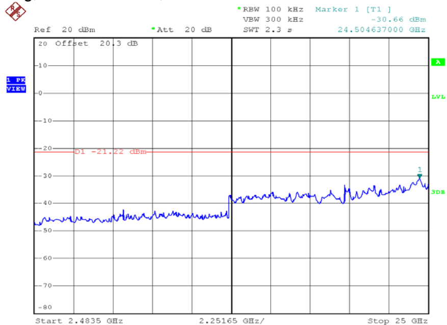
802.11g, Lowest Channel, Plot B
