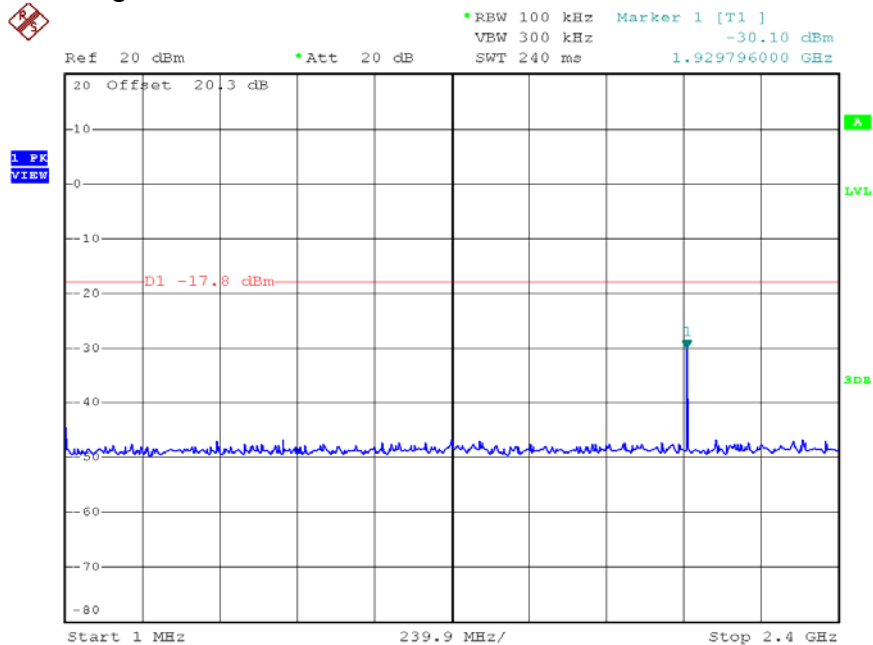
802.11b, Highest Channel, Plot A
