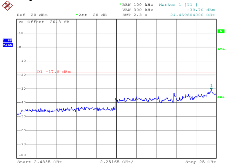
802.11b, Highest Channel, Plot B
