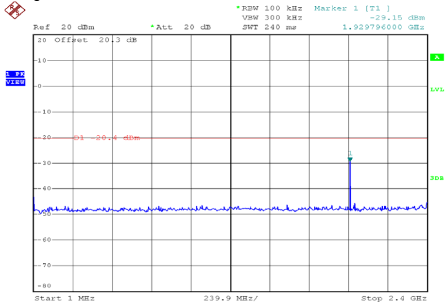
802.11g, Middle Channel, Plot A
