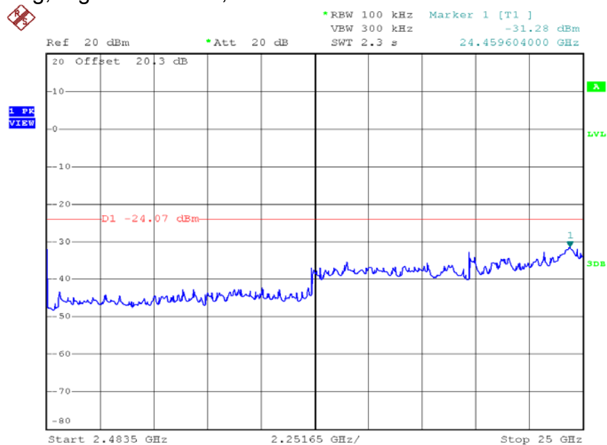
802.11g, Highest Channel, Plot B
