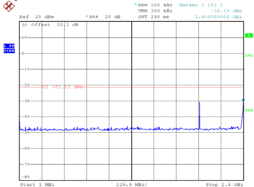
802.11g, Lowest Channel, Plot A
