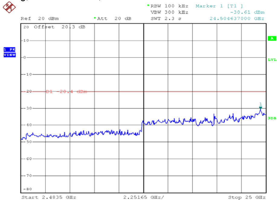
802.11g, Middle Channel, Plot B
