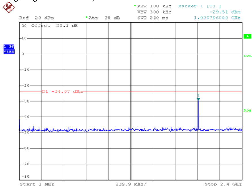
802.11g, Highest Channel, Plot A
