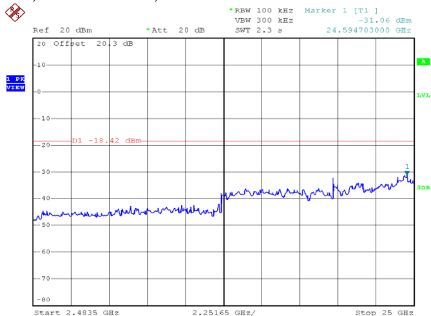
802.11b, Lowest Channel, Plot B
