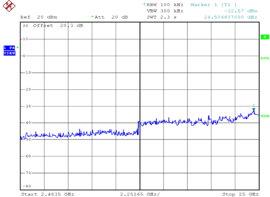
802.11b, Middle Channel, Plot B
